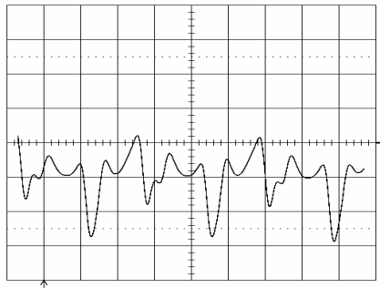
Output voltage ripple (20mV/div.) at: T_{ref} = +25^\circ\text{C} , I_O = 30\text{ A} resistive load, V_i = 5.0\text{ V} . Time scale: 2 \mu\text{s}/\text{div} . See the filter in the Output ripple and noise section (EMC Specification).
