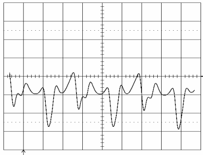
Output voltage ripple (20mV/div.) at: T_{ref} = +25^\circ\text{C} , I_O = 30\text{ A} resistive load, V_i = 5.0\text{ V} . Time scale: 2 \mu\text{s}/\text{div} . See the filter in the Output ripple and noise section (EMC Specification).
