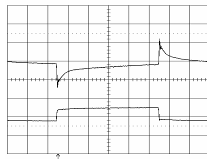
Output voltage response to load current step- change (15-30-15 A) at: T_{ref} = +25^\circ\text{C} , V_i = 5.0\text{ V} . Top trace: output voltage (100mV/div.). Bottom trace: load current (20 A/div.). Time scale: 0.1 ms/div..
