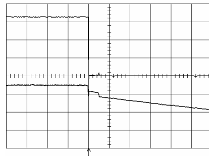
Shut-down enabled by disconnecting V_i at: T_{ref} = +25^\circ\text{C} , I_O = 30\text{ A} resistive load, V_i = 5.0\text{ V} . Top trace: output voltage (1.0 V/div.). Bottom trace: input voltage (2 V/div.). Time scale: 5.0 ms/div..
