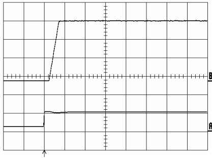
Start-up enabled by connecting V_i at: T_{ref} = +25^\circ\text{C} , I_O = 30\text{ A} resistive load, V_i = 5.0\text{ V} . Top trace: output voltage (1.0 V/div.). Bottom trace: input voltage (5 V/div.). Time scale: 10 ms/div..
