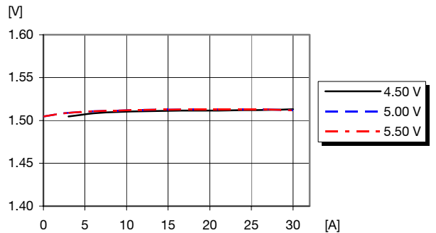
Output voltage vs. load current at T_{ref} = +25^{\circ}C
