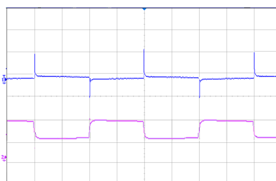
Figure 5 Dynamic response for 25% load step (25% ~ 50% ~ 25%) and 1A/µs slew rate, (2ms/div), see Figure 11 for test configuration; CH1-output voltage (50mV/div); CH2-output current (10A/div)
