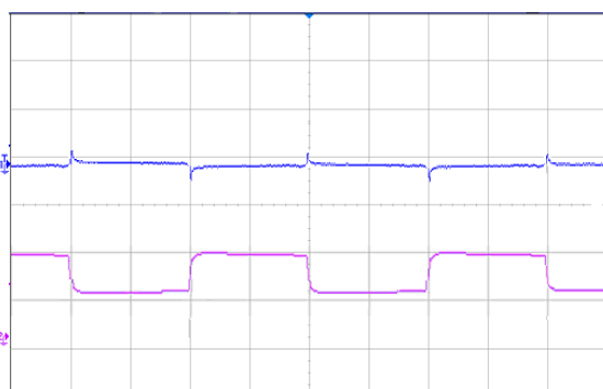
Figure 4 Dynamic response for 25% load step (25% ~ 50% ~ 25%) and 0.1A/µs slew rate, (2ms/div), see Figure 11 for test configuration; CH1-output voltage (50mV/div); CH2-output current (10A/div)
