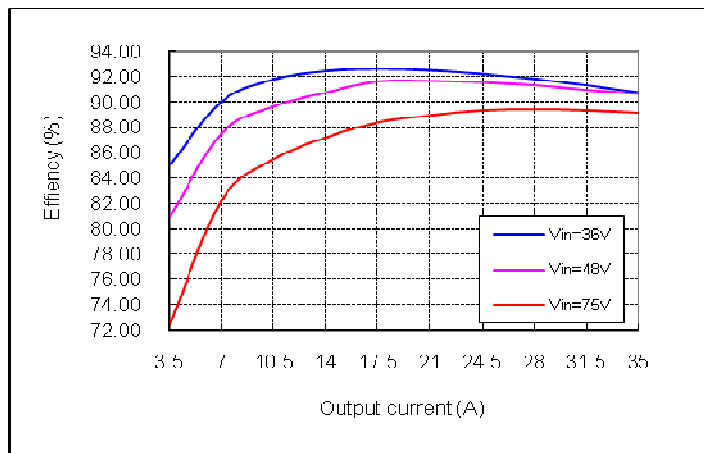
Figure 1 Efficiency vs. output current, Ta = 25°C, Vo = 2.5V, Air velocity = 300LFM
