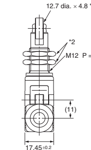
*1. Stainless-steel roller *2. Two hexagonal nuts (3 t × 17 width across flats)
