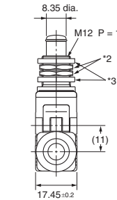
* Stainless-steel plunger
