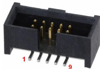
Figure 28: JTAG Connector
