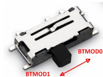
Figure 2: BMD Switch
