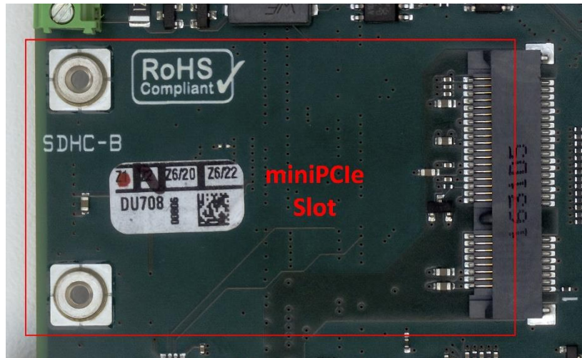
Figure 33: miniPCIe Slot
