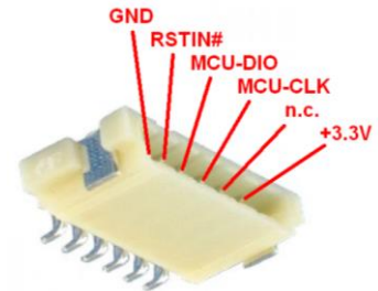
Figure 20: Module MCU Connector
