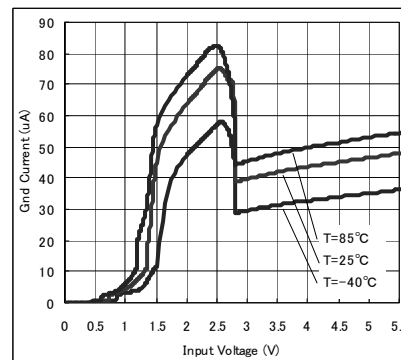
Fig.26 Circuit Current
