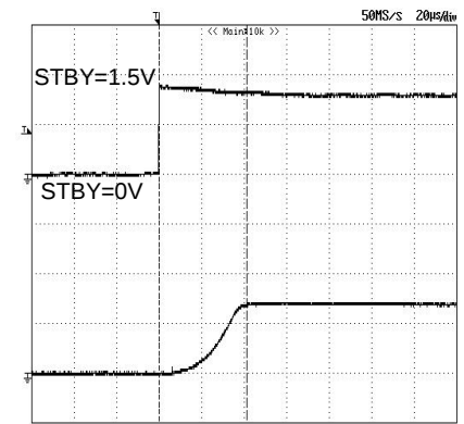
Fig.40 START_UP (Ta=85°C)
