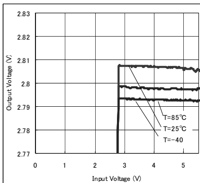
Fig.25 Line Regulation
