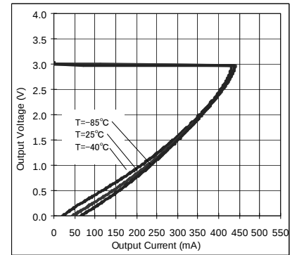
Fig.52 OCP Threshold
