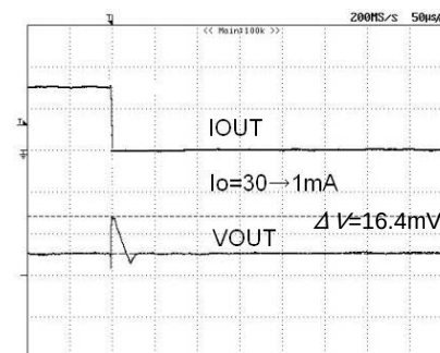
Fig.46 Load_response (Io=30→1mA) (Ta=25°C)
