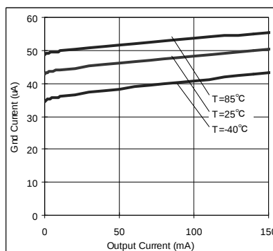
Fig.28 IOU - IGND
