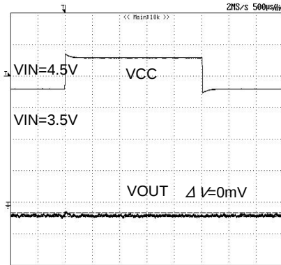
Fig.35 Transient_response (Ta=-40°C)
