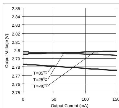
Fig.27 Load Regulation
