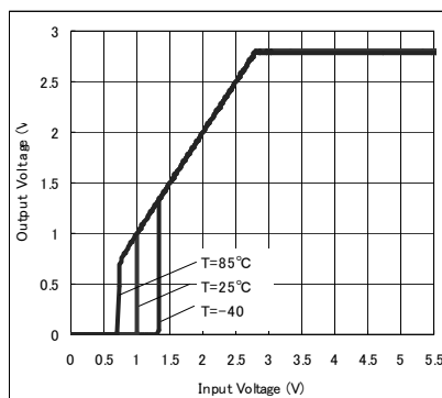
Fig.24 Output Voltage
