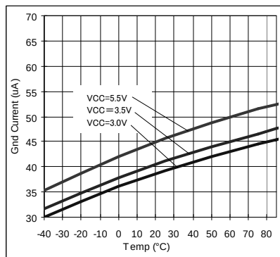
Fig.54 IGND - Temp
