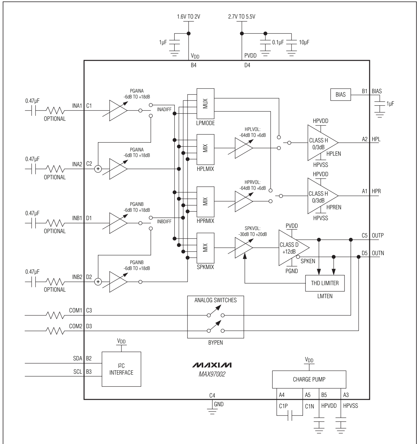
Functional Diagram/Typical Application Circuit
