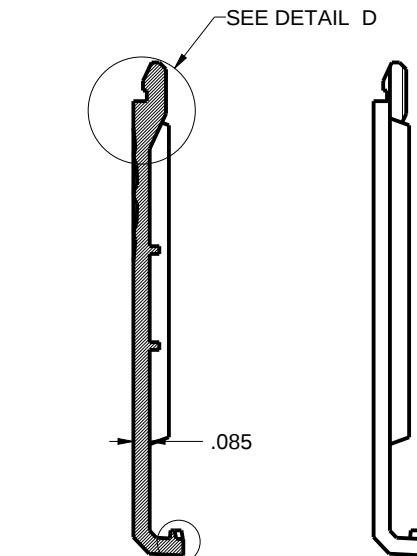
SECTION X-X
