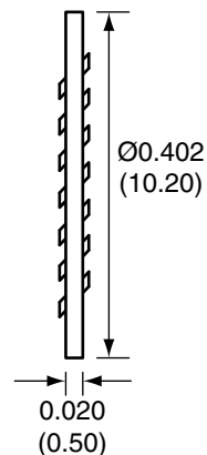
WASHER
