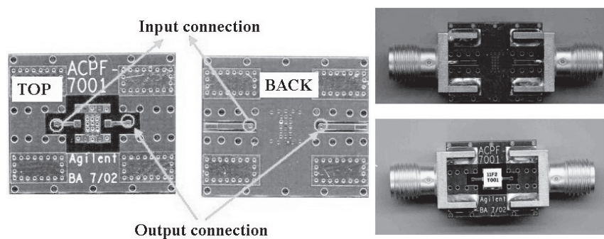
Figure 6. PCB top and bottom views (vias used to connect the underside of the board to the filter mounting pads on top).
