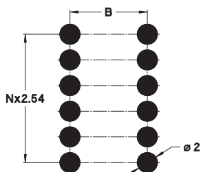
PCB LAYOUT
