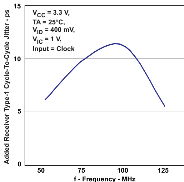
ADDED RECEIVER TYPE-1 CYCLE-TO-CYCLE JITTER vs FREQUENCY
