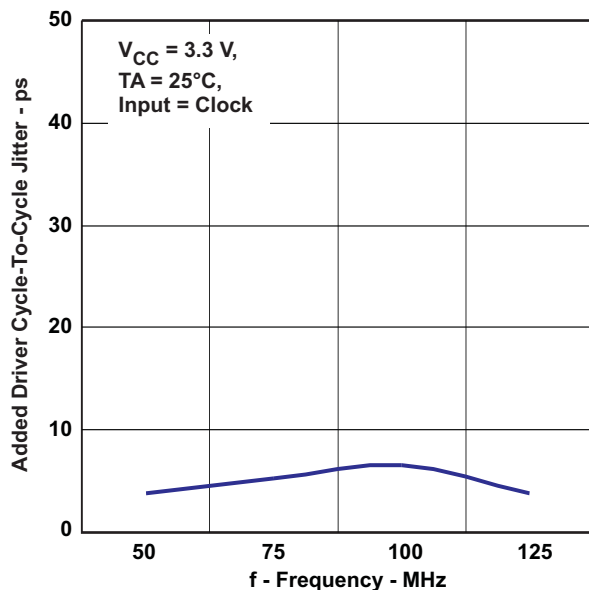
ADDED DRIVER CYCLE-TO-CYCLE JITTER vs FREQUENCY
