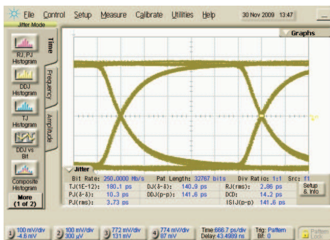
DRIVER OUTPUT EYE PATTERN 250 Mbps, 2^{15}-1 PRBS, V_{CC} = 3.3 \text{ V}
