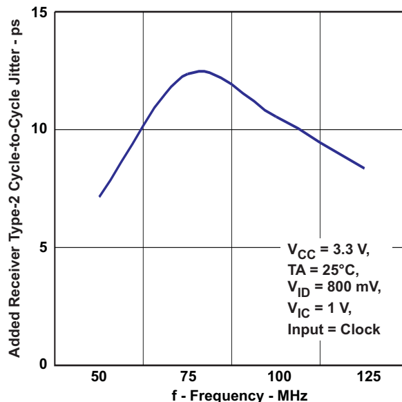
ADDED RECEIVER TYPE-2 CYCLE-TO-CYCLE JITTER vs FREQUENCY
