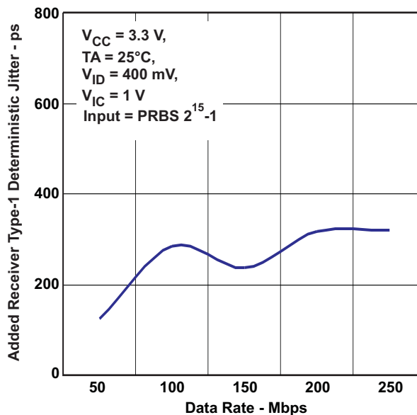
ADDED RECEIVER TYPE-1 DETERMINISTIC JITTER vs DATA RATE
