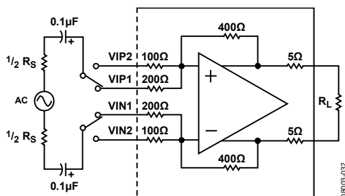
Figure 32. Basic Structure
