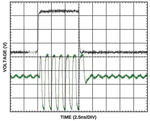
Figure 22. ENBL Time Domain Response
