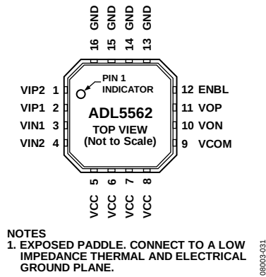
Figure 2. Pin Configuration
