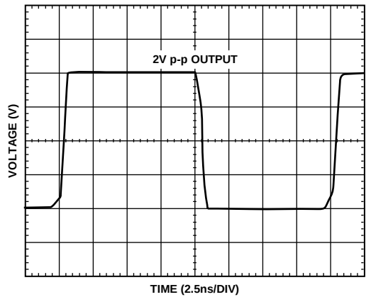
Figure 23. Large Signal Pulse Response, A_V = 15.5 dB
