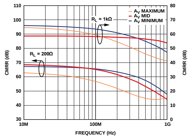
Figure 26. Common-Mode Rejection Ratio (CMRR) vs. Frequency
