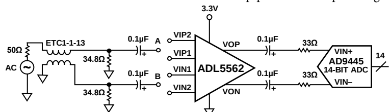
Figure 39. Wideband ADC Interfacing Example Featuring the AD9445
