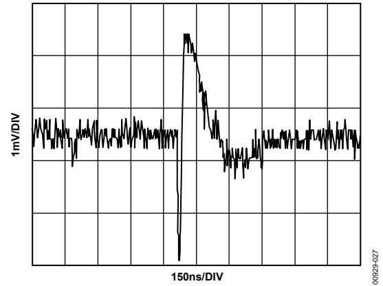
Figure 27. DAC-to-DAC Crosstalk
