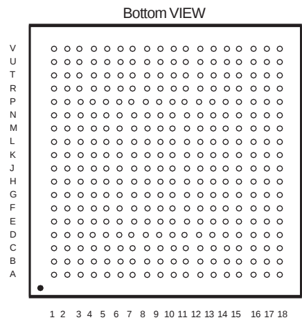
Figure 4-1. Orientation of the 324-ball LFBGA Package
