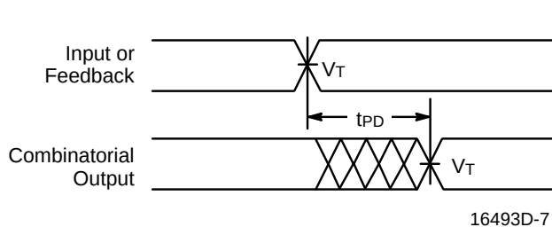
Combinatorial Output
