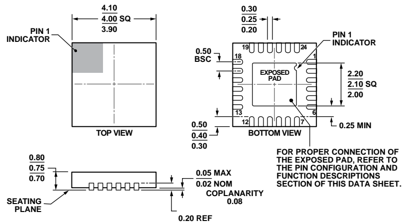
Figure 54. 24-Lead Lead Frame Chip Scale Package [LFCSP_WQ]
