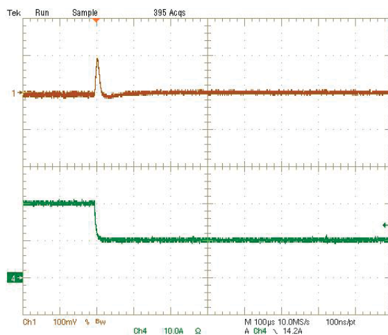
Step Load Transient Response (Vin=12V, Vout=2.5V, Cloud=188µF, Iout=20A to 10A) Trace 1=Vout, 100 mV/div(AC), Trace 4=Iout, 10A/div.
