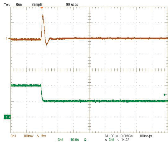
Step Load Transient Response (Vin=7V, Vout=0.69V, Cload=188µF, Iout=20A to 10A) Trace 1=Vout, 100 mV/div(AC), Trace 4=Iout, 10A/div.
