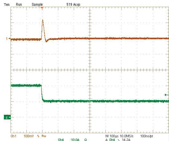
Step Load Transient Response (Vin=12V, Vout=1.2V, Cload=188µF, Iout=20A to 10A) Trace 1=Vout, 100 mV/div(AC), Trace 4=Iout, 10A/div.
