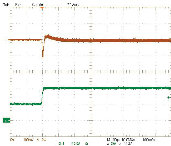
Step Load Transient Response (Vin=12V, Vout=5.0V, Cload=188µF, Iout=10A to 20A) Trace 1=Vout, 100 mV/div(AC), Trace 4=Iout, 10A/div.
