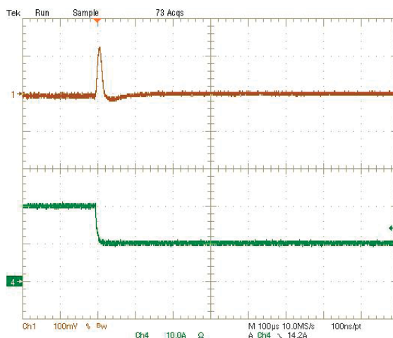
Step Load Transient Response (Vin=12V, Vout=1.8V, Cload=188µF, Iout=20A to 10A) Trace 1=Vout, 100 mV/div(AC), Trace 4=Iout, 10A/div.
