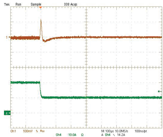
Step Load Transient Response (Vin=12V, Vout=5.0V, Cload=188µF, Iout=20A to 10A) Trace 1=Vout, 100 mV/div(AC), Trace 4=Iout, 10A/div.
