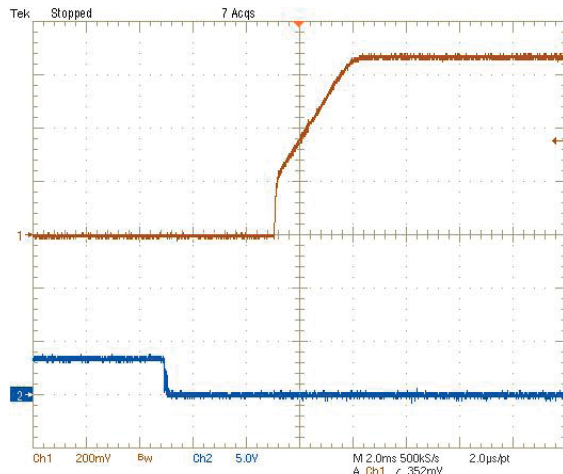
On/Off Enable Delay (Vin=5.5V, Vout=0.69V, Iout=20A, Cload=188µF) Trace2=Enable, 5v/div, Trace1=Vout,200mV/div
