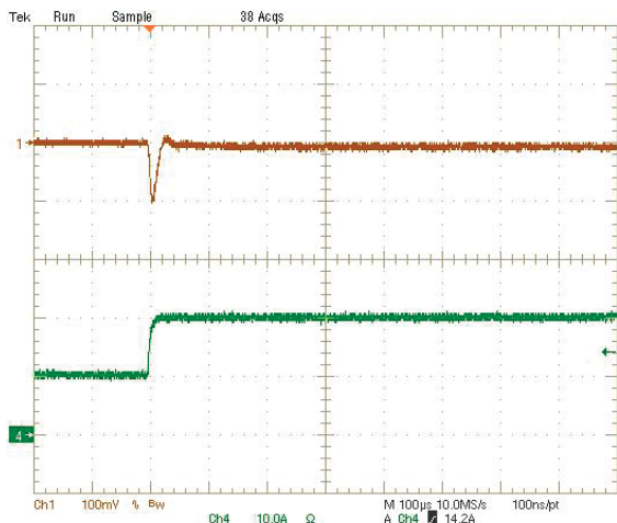
Step Load Transient Response (Vin=12V, Vout=1.2V, Cload=188µF, Iout=10A to 20A) Trace 1=Vout, 100 mV/div(AC), Trace 4=Iout, 10A/div.
