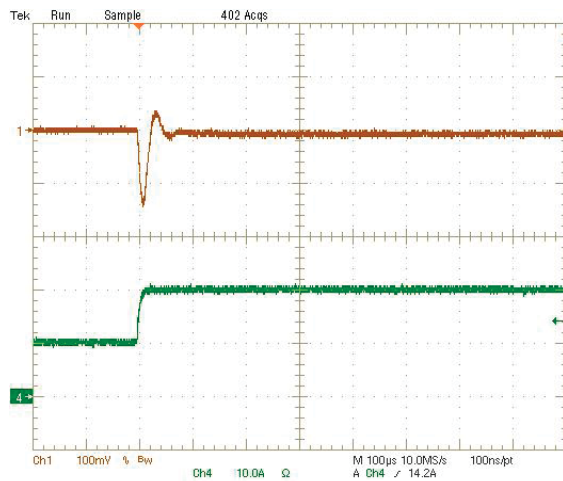
Step Load Transient Response (Vin=7V, Vout=0.69V, Cload=188µF, Iout=10A to 20A) Trace 1=Vout, 100 mV/div(AC), Trace 4=Iout, 10A/div.
