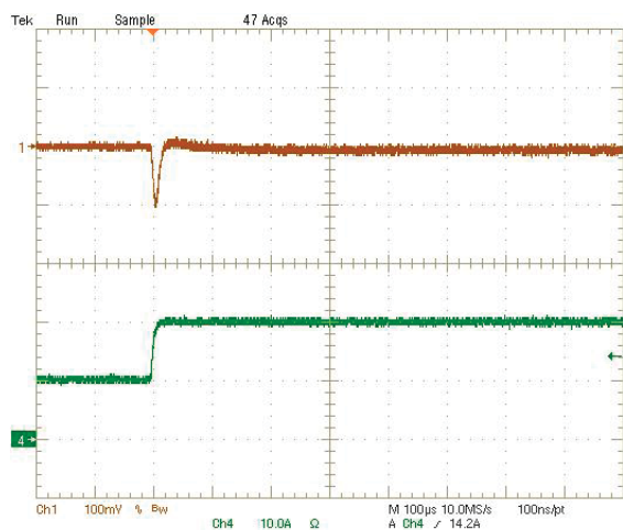
Step Load Transient Response (Vin=12V, Vout=2.5V, Cloud=188µF, Iout=10A to 20A) Trace 1=Vout, 100 mV/div(AC), Trace 4=Iout, 10A/div.
