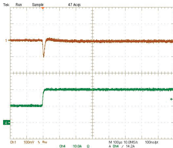
Step Load Transient Response (Vin=12V, Vout=2.5V, Cloud=188μF, Iout=10A to 20A) Trace 1=Vout, 100 mV/div(AC), Trace 4=Iout, 10A/div.
