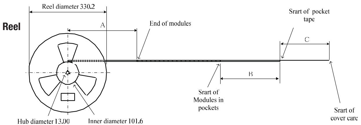
Reel Information (200 units per reel)
