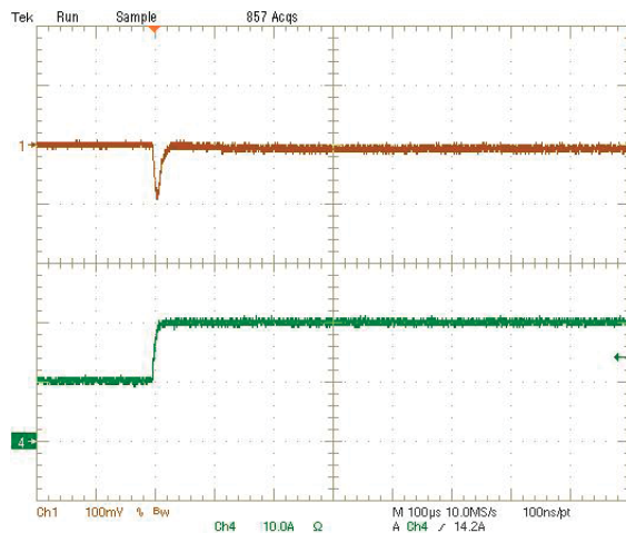
Step Load Transient Response (Vin=12V, Vout=1.8V, Cload=188µF, Iout=10A to 20A) Trace 1=Vout, 100 mV/div(AC), Trace 4=Iout, 10A/div.
