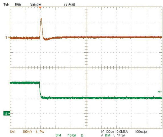
Step Load Transient Response (Vin=12V, Vout=1.8V, Cload=188µF, Iout=20A to 10A) Trace 1=Vout, 100 mV/div(AC), Trace 4=Iout, 10A/div.
