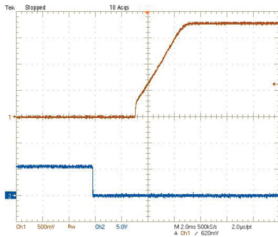
On/Off Enable Delay (Vin=12V, Vout=1.8V, Iout=20A, Cload=188µF) Trace2=Enable, 5V/div Trace1=Vout, 500mV/div
