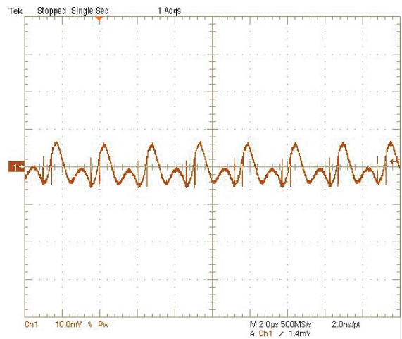
Output Ripple and Noise (Vin=12V, Vout=1.8V, Iout=20A, Cload=188µF, ScopeBW=20MHz) Trace1=Vout, 10mV/div(AC)
