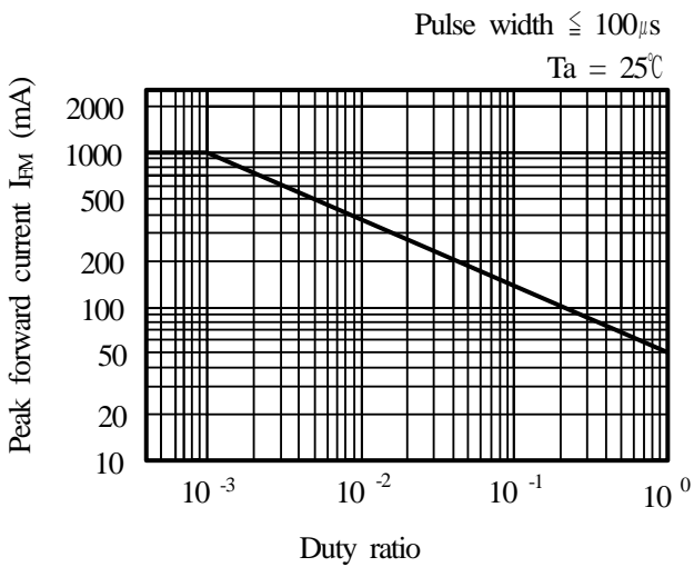
(Fig.7) Forward current vs. duty ratio
