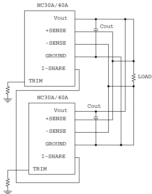
Figure 30: NC30/NC40 Current Sharing Diagram
