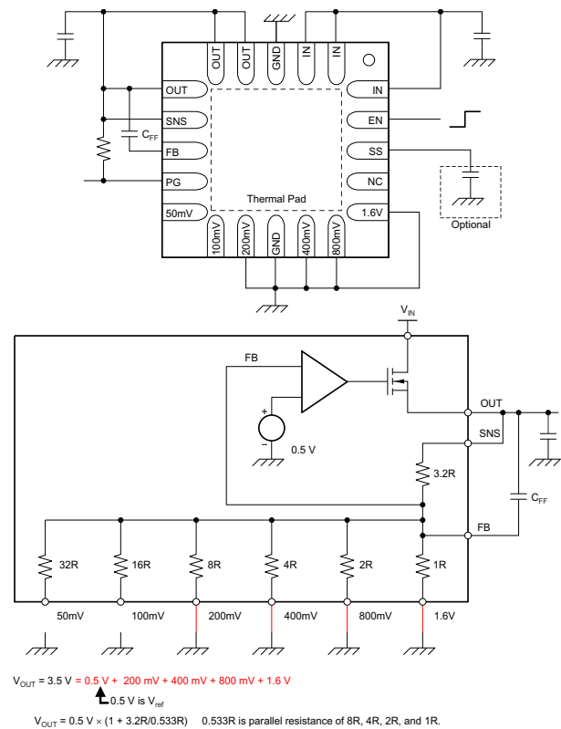
Figure 39. 3.5-V Configuration
