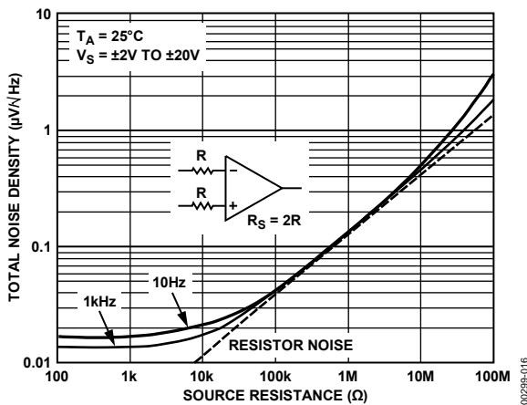
Figure 16. Total Noise Density vs. Source Resistance
