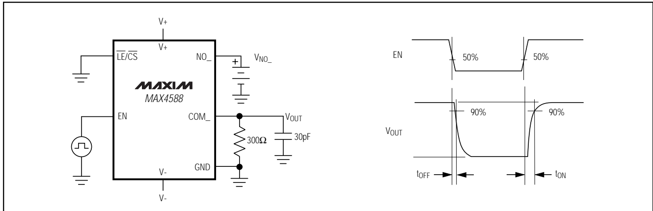
Figure 1. Turn-On/Turn-Off Time
