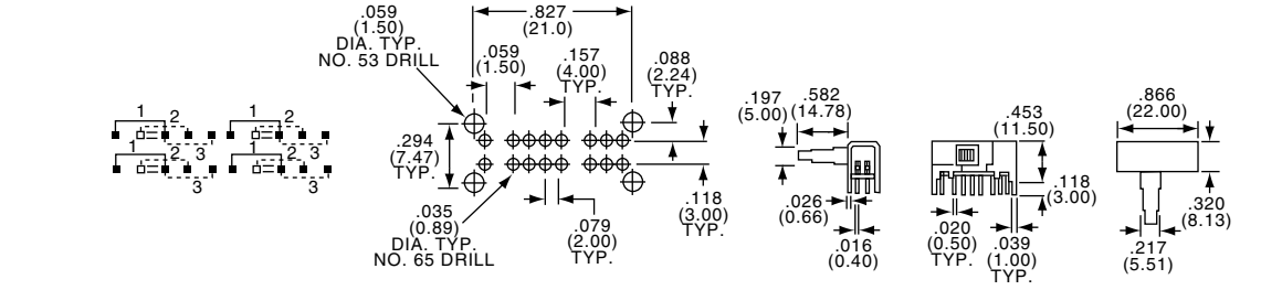
MSS4350R
