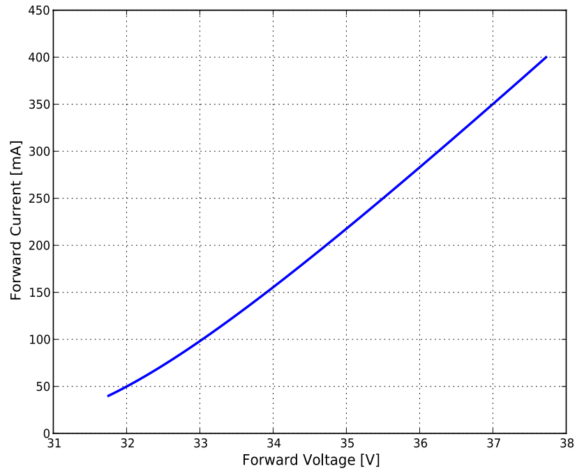
Figure 4c. Typical forward current vs. forward voltage for L2C3-xxxx209E06000 at T j =85°C.
