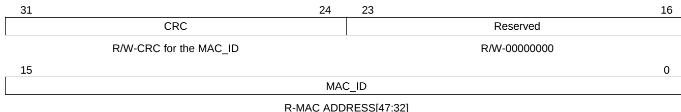
Figure 3-12. MAC_ADDR_RW1 Register
