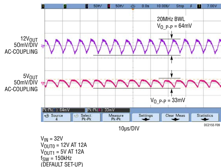
Figure 9. DC2155A-A Output Ripple Voltages
