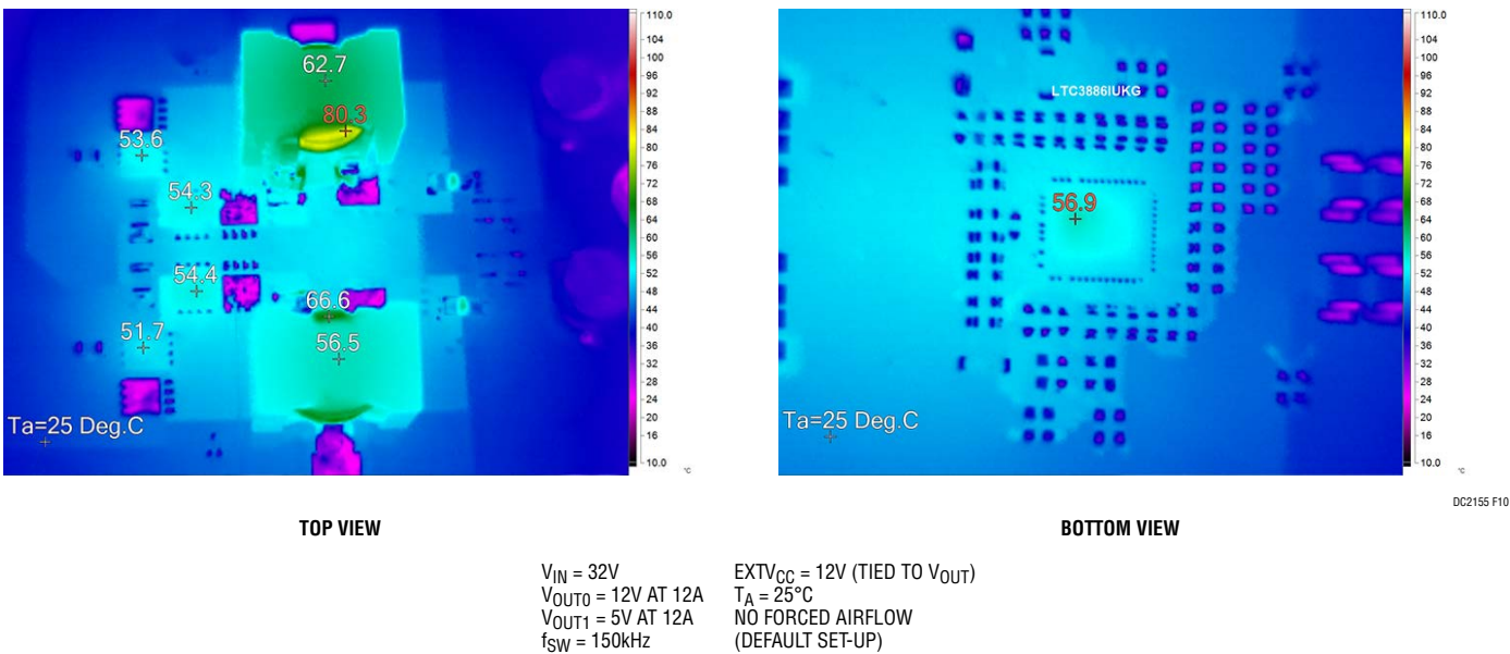
Figure 10. DC2155A-A Thermal Performance
