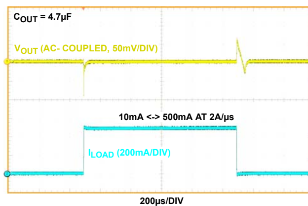
FIGURE 21. LOAD TRANSIENT RESPONSE
