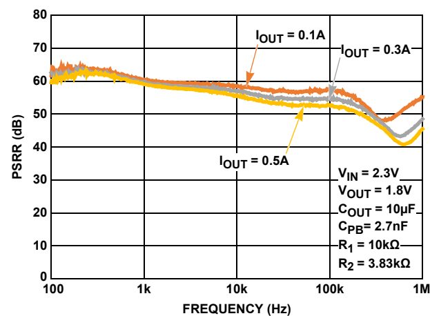
FIGURE 2. PSRR
