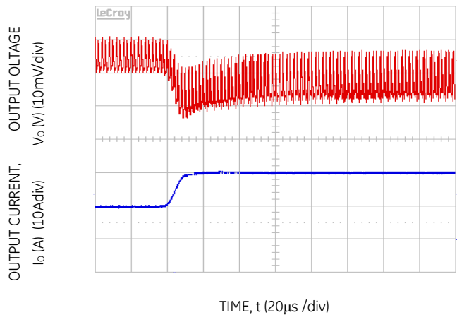
Figure 4. Transient Response to Dynamic Load Change from 50% to 100% at 12Vin, C out = 1x47µF +11x330µF CTune=47nF, RTune=178 ohms
