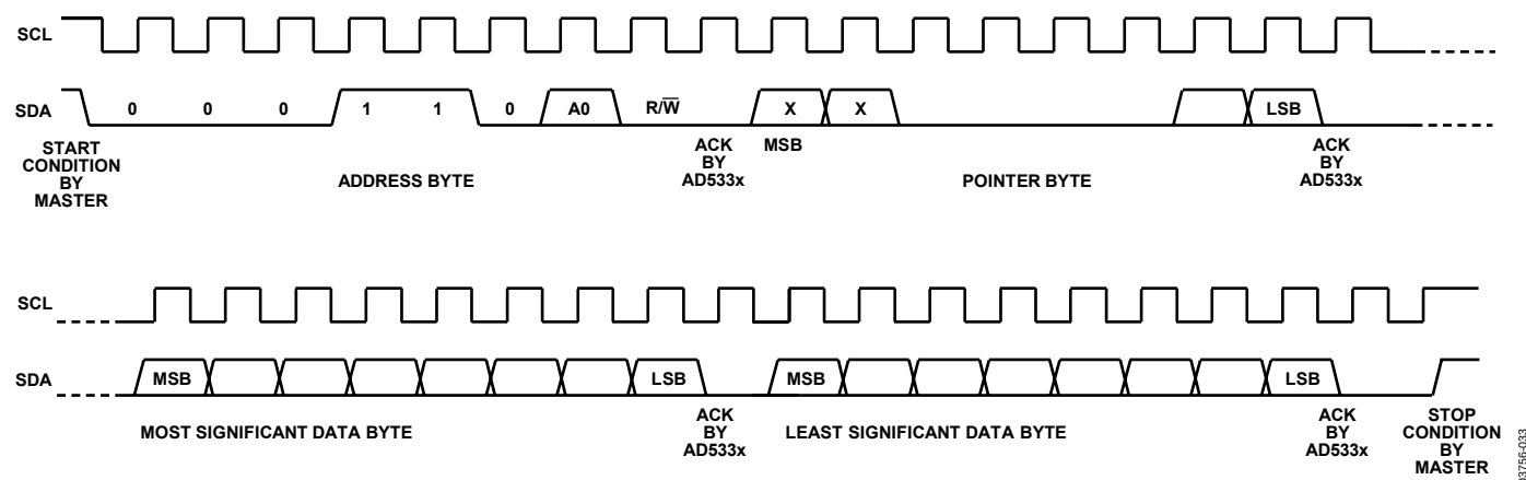
Figure 33. Write Sequence
