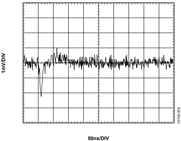
Figure 26. DAC-to-DAC Crosstalk
