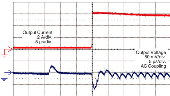
Transient Response in Power Save Mode (0.2 A - 6 A) (V_{IN} = 12\text{ V}, V_{OUT} = 1\text{ V}, F_{SW} = 500\text{ kHz at } 6\text{ A})
