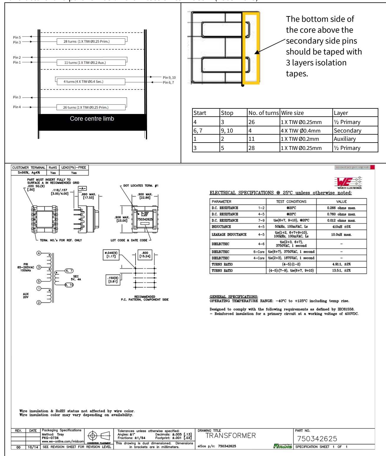
Figure 5 Transformer structure
