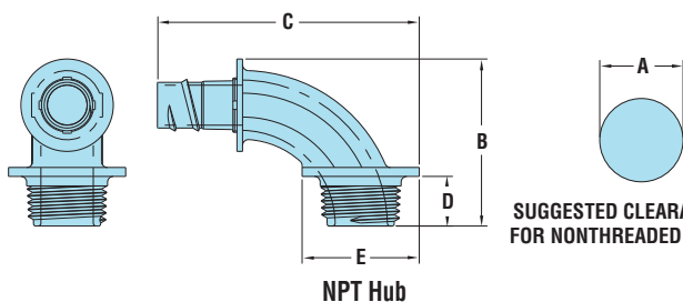
NPT Hub
