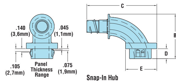
Snap-In Hub
