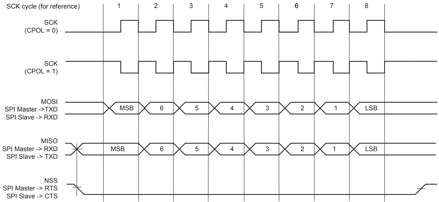
Figure 44-36. SPI Transfer Format (CPHA = 1, 8 bits per transfer)
