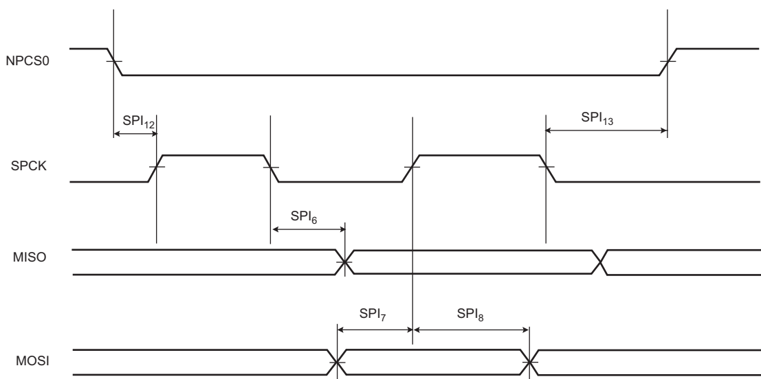
Figure 56-29. USART SPI Slave Mode 1 or 2
