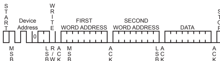
Figure 40-14. Internal Address Usage
