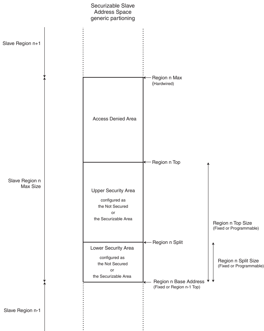
Figure 16-1. Generic Partitioning of the AHB Slave Address Space
