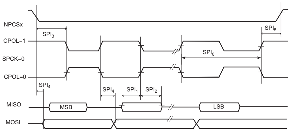
Figure 56-28. USART SPI Master Mode
