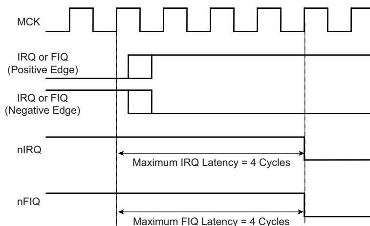
Figure 18-6. External Interrupt Edge Triggered Source
