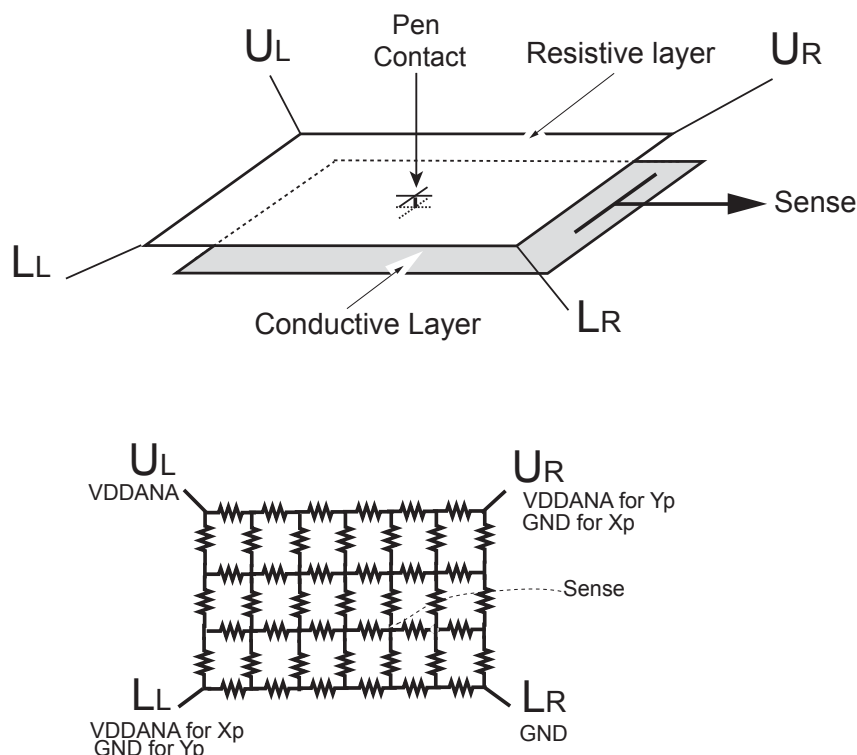
Figure 48-12. 5-Wire Principle
