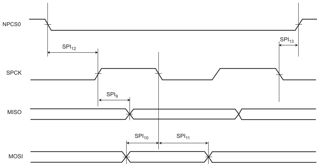
Figure 56-11. SPI Slave Mode 1 and 2
