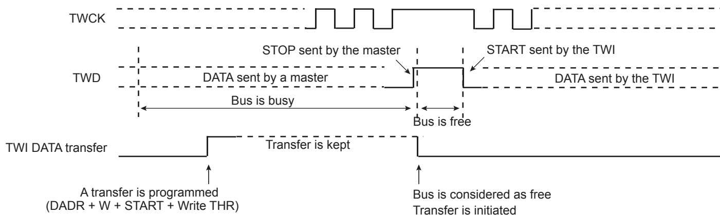
Figure 40-21. Programmer Sends Data While the Bus is Busy
