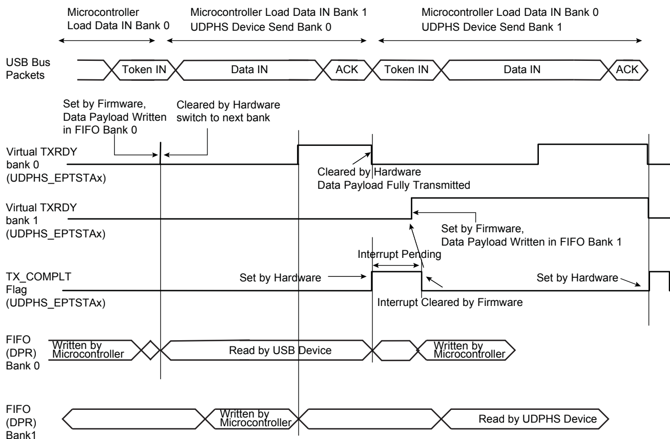
Figure 35-10. Data IN Transfer for Endpoint with Two Banks
