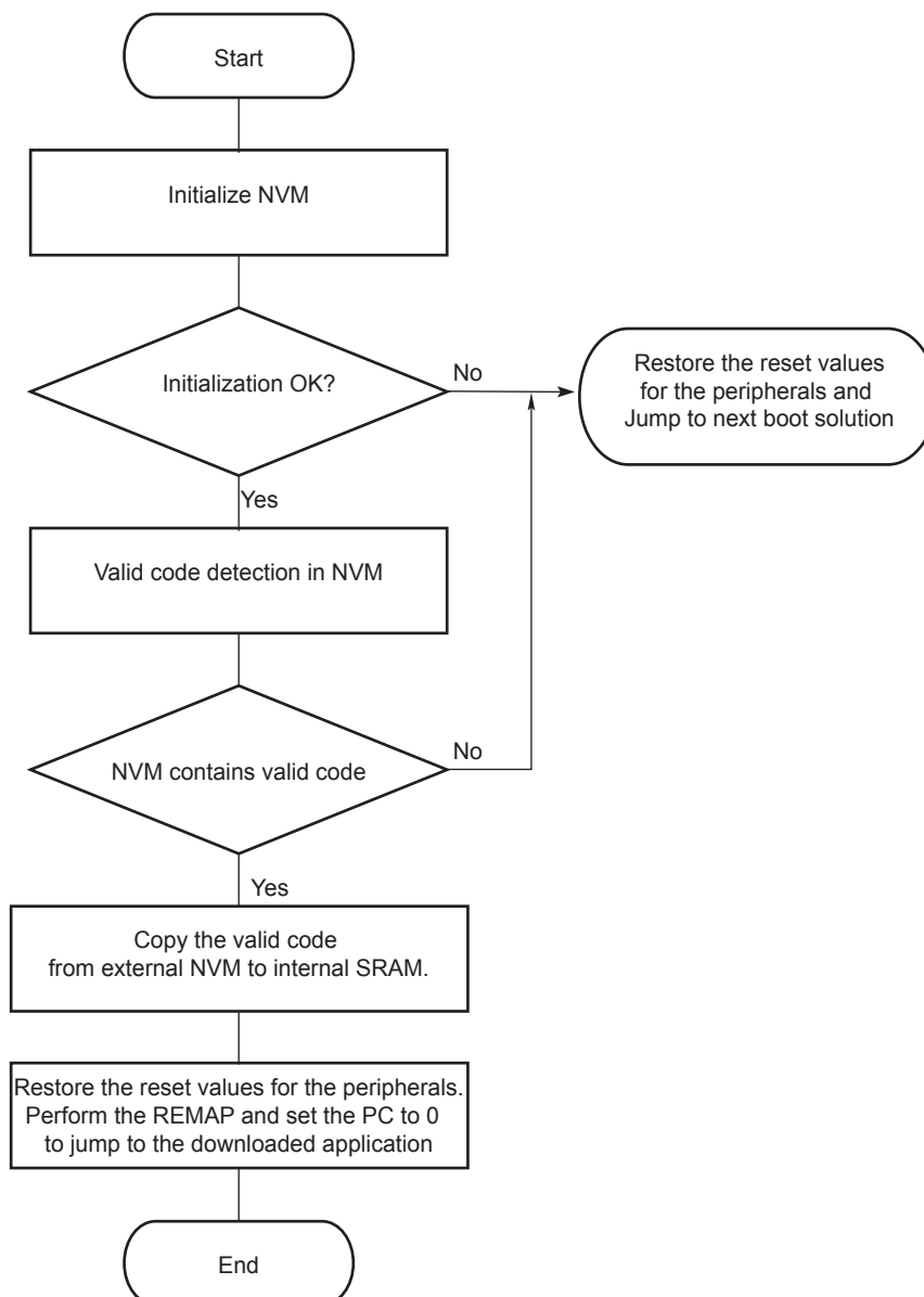
Figure 13-3. NVM Bootloader Program Diagram
