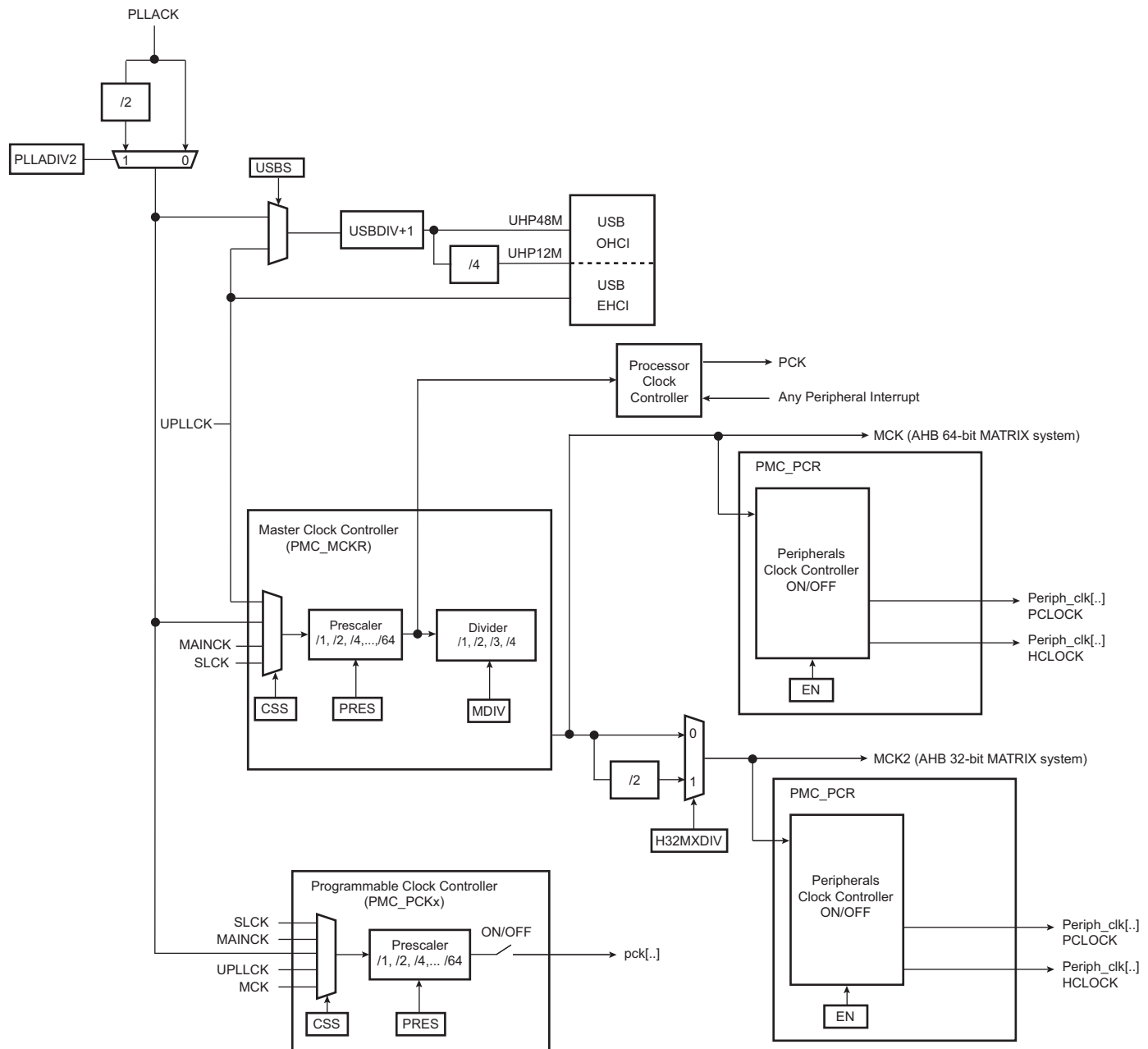
Figure 27-1. General Clock Block Diagram
