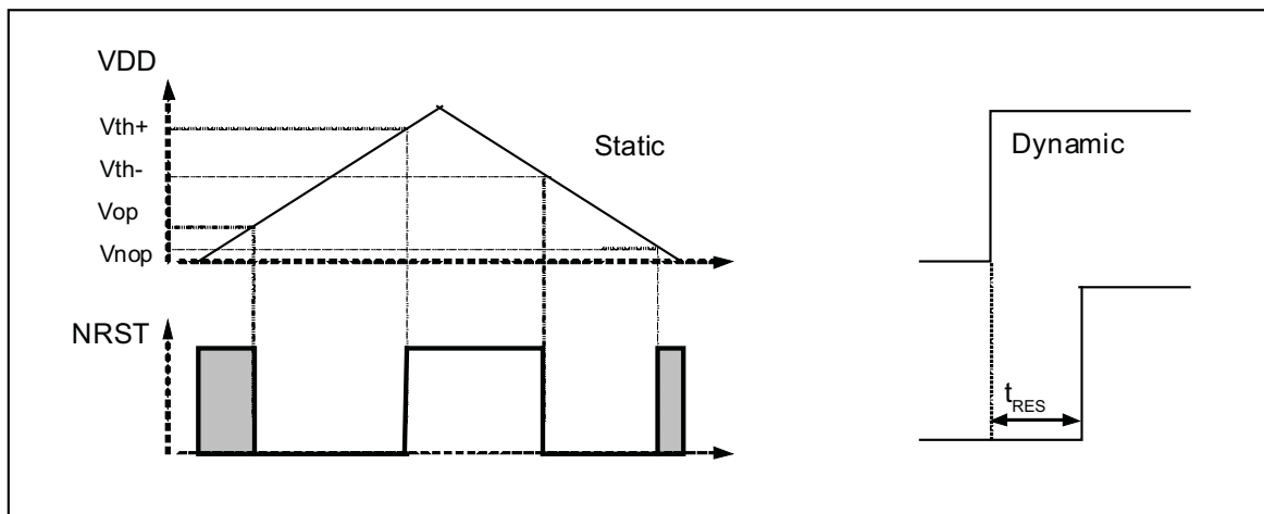
Figure 56-5. General Presentation of POR Behavior
