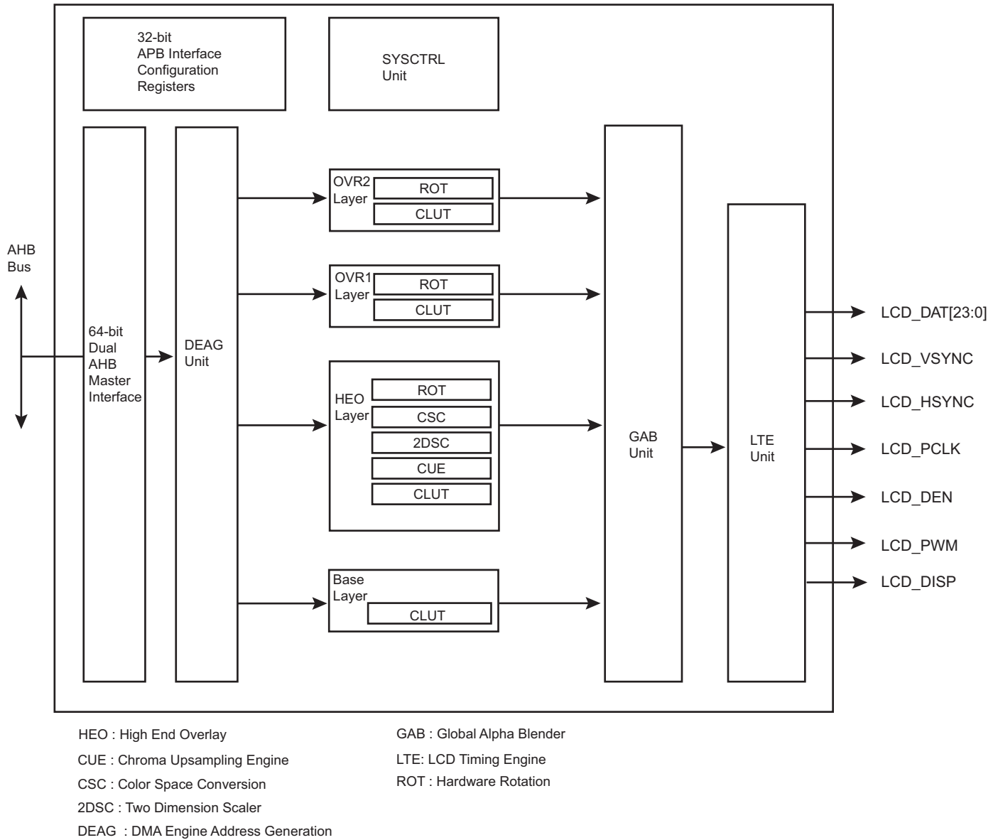
Figure 32-1. Block Diagram
