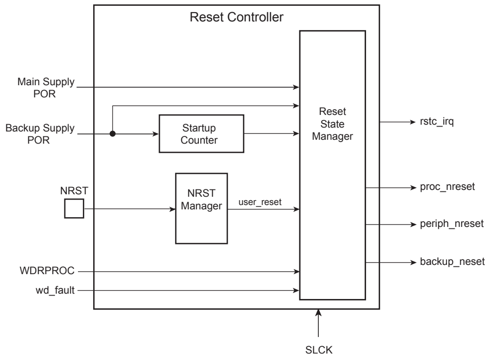
Figure 20-1. Reset Controller Block Diagram
