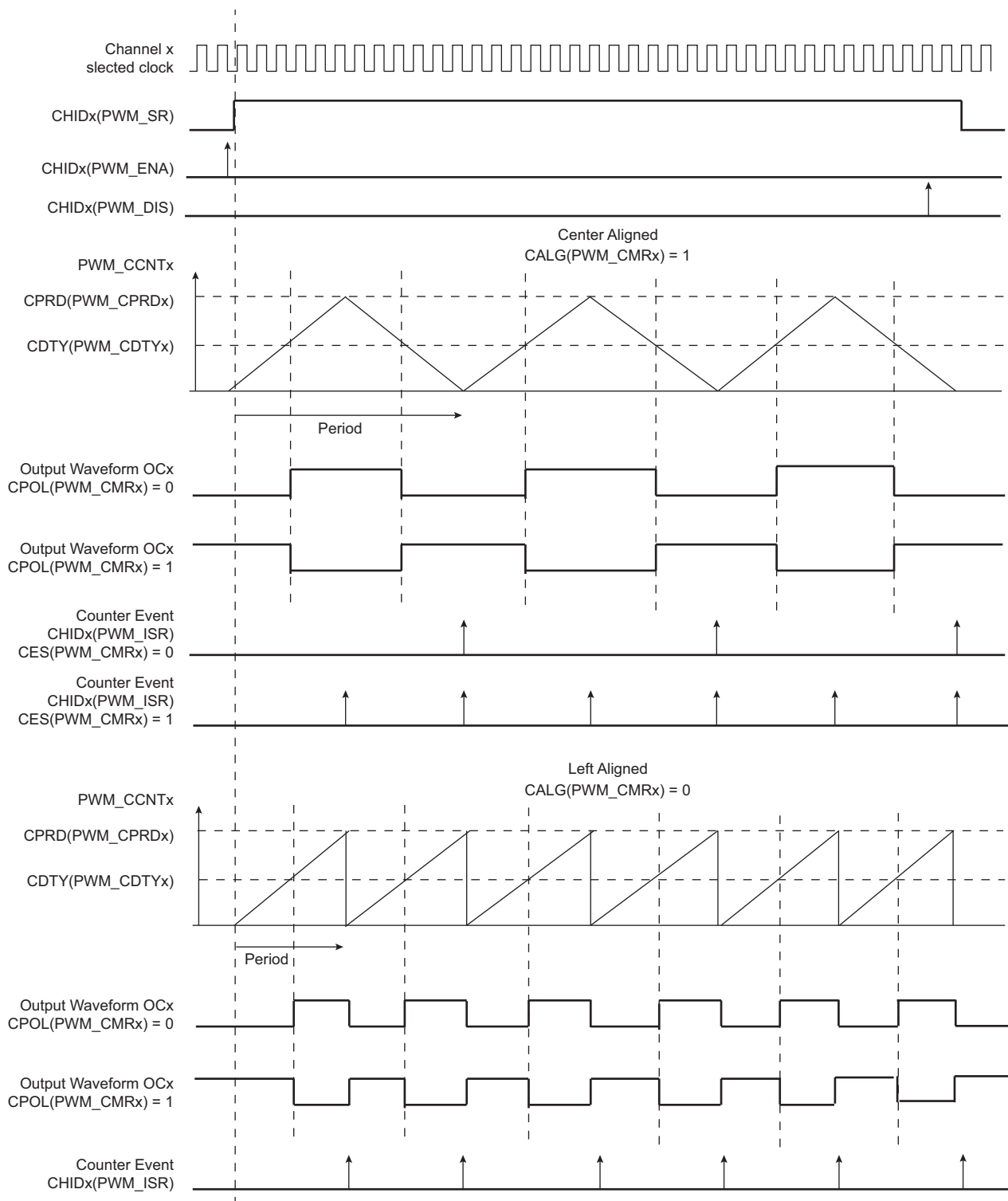
Figure 47-5. Waveform Properties
