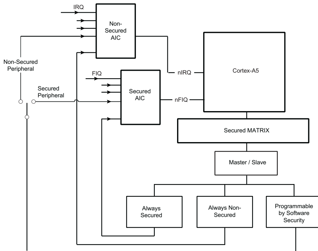
Figure 18-3. AIC Detailed Block Diagram
