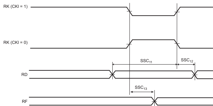
Figure 56-21. SSC Receiver, RK and RF in Output
