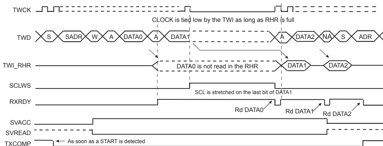
Figure 40-29. Clock Synchronization in Write Mode
