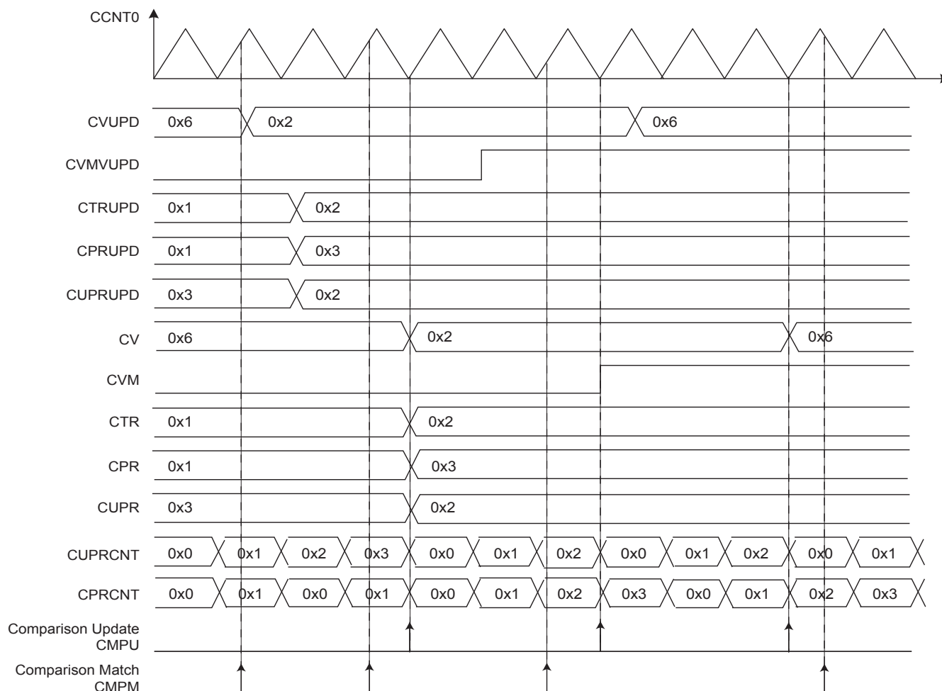
Figure 47-16. Comparison Waveform
