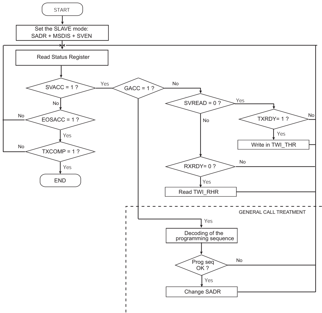
Figure 40-32. Read Write Flowchart in Slave Mode
