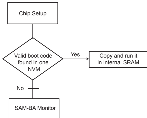
Figure 13-1. ROM Code Algorithm Flow Diagram
