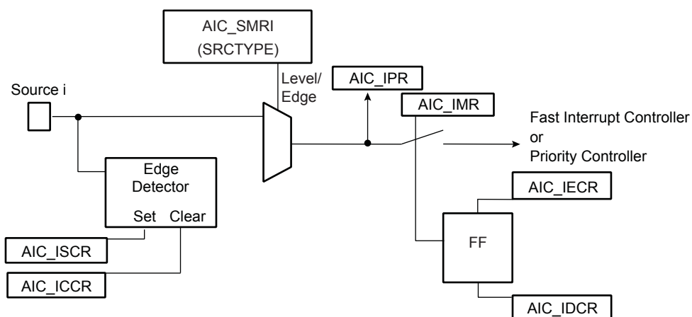
Figure 18-4. Internal Interrupt Source Input Stage
