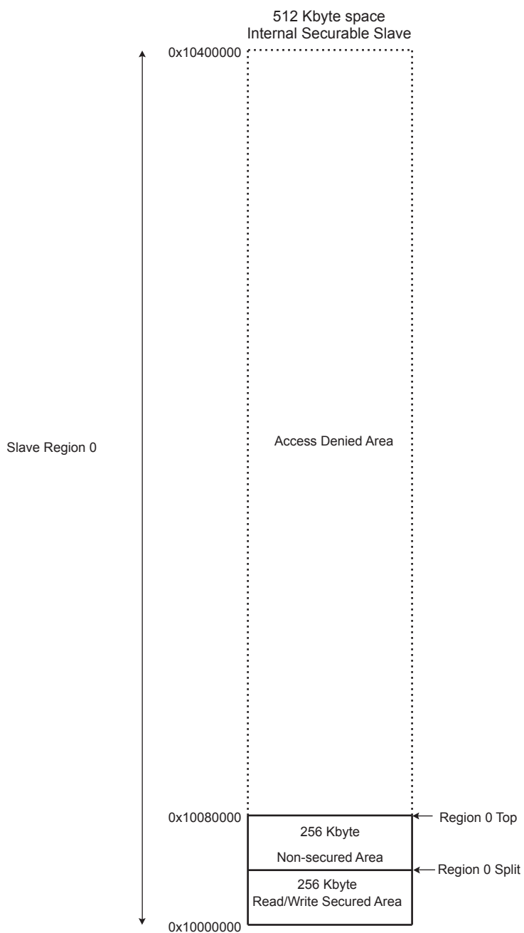
Figure 16-2. Partitioning example of an Internal Securable slave featuring 1 security region of 512 KB split into 1 or 2 security areas of 4 KB to 512 KB
