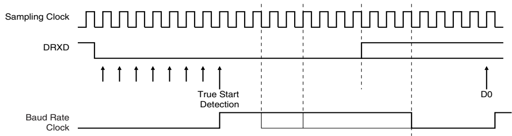
Figure 42-4. Start Bit Detection
