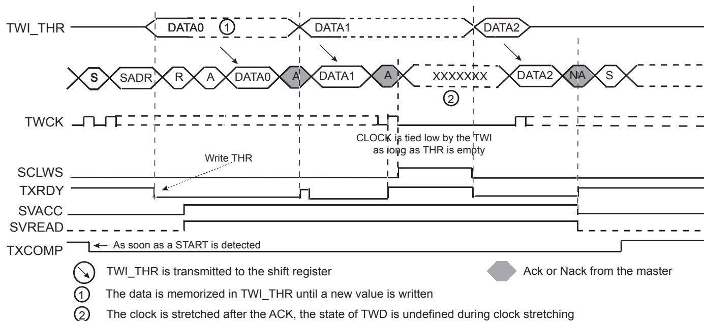
Figure 40-28. Clock Stretching in Read Mode
