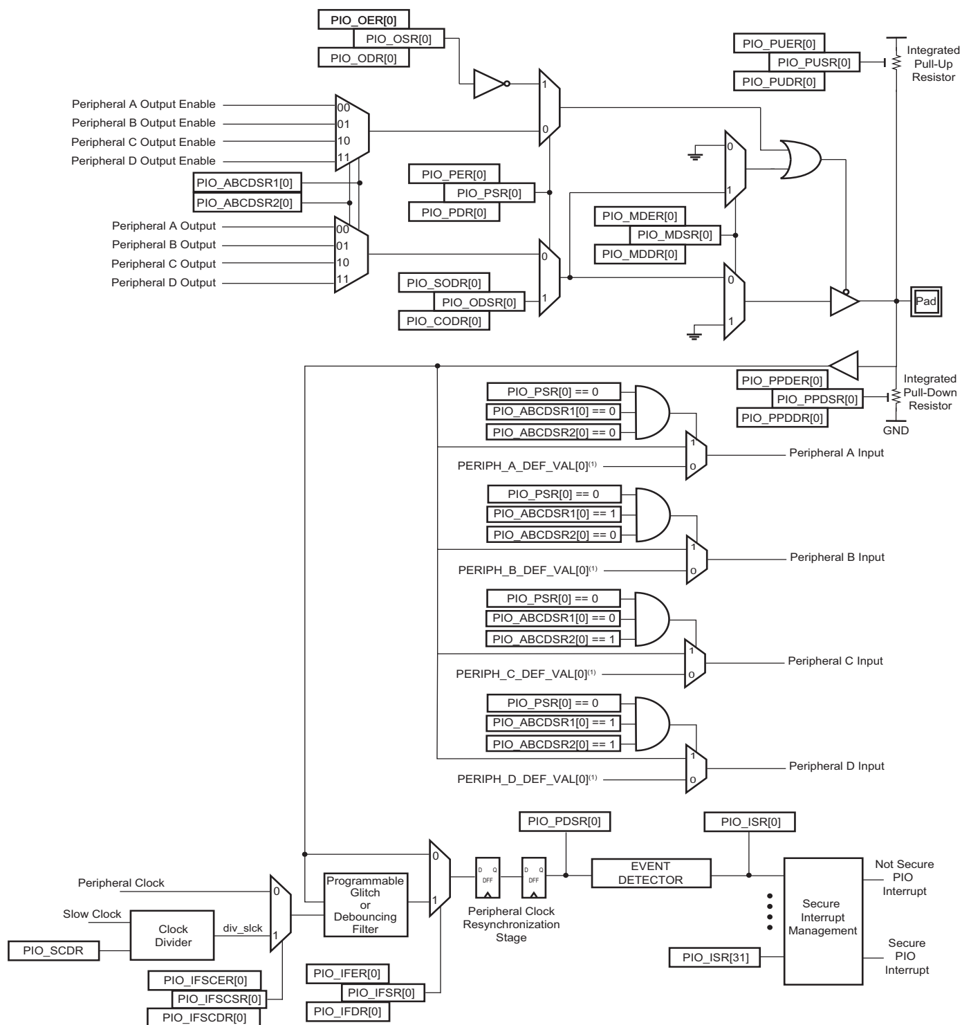
Figure 28-2. I/O Line Control Logic
