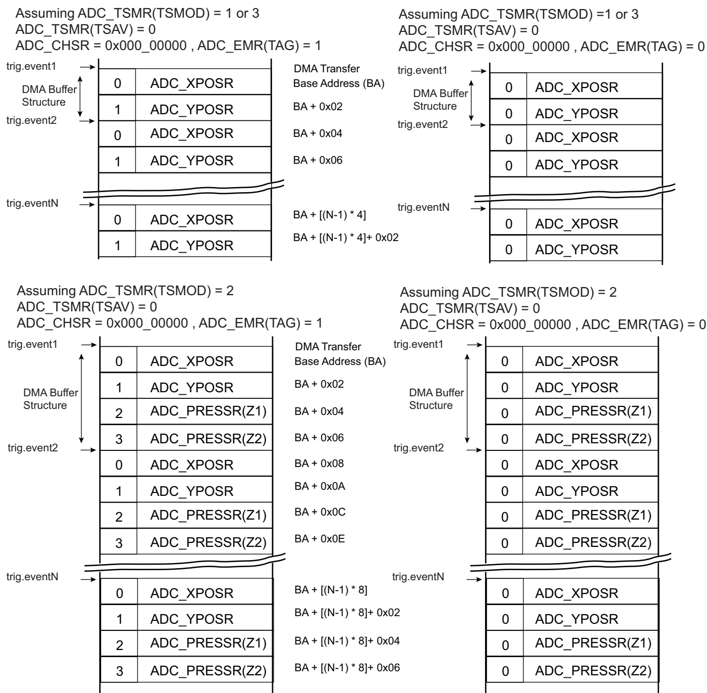
Figure 48-17. Buffer Structure When Only Touchscreen Channels are Enabled
