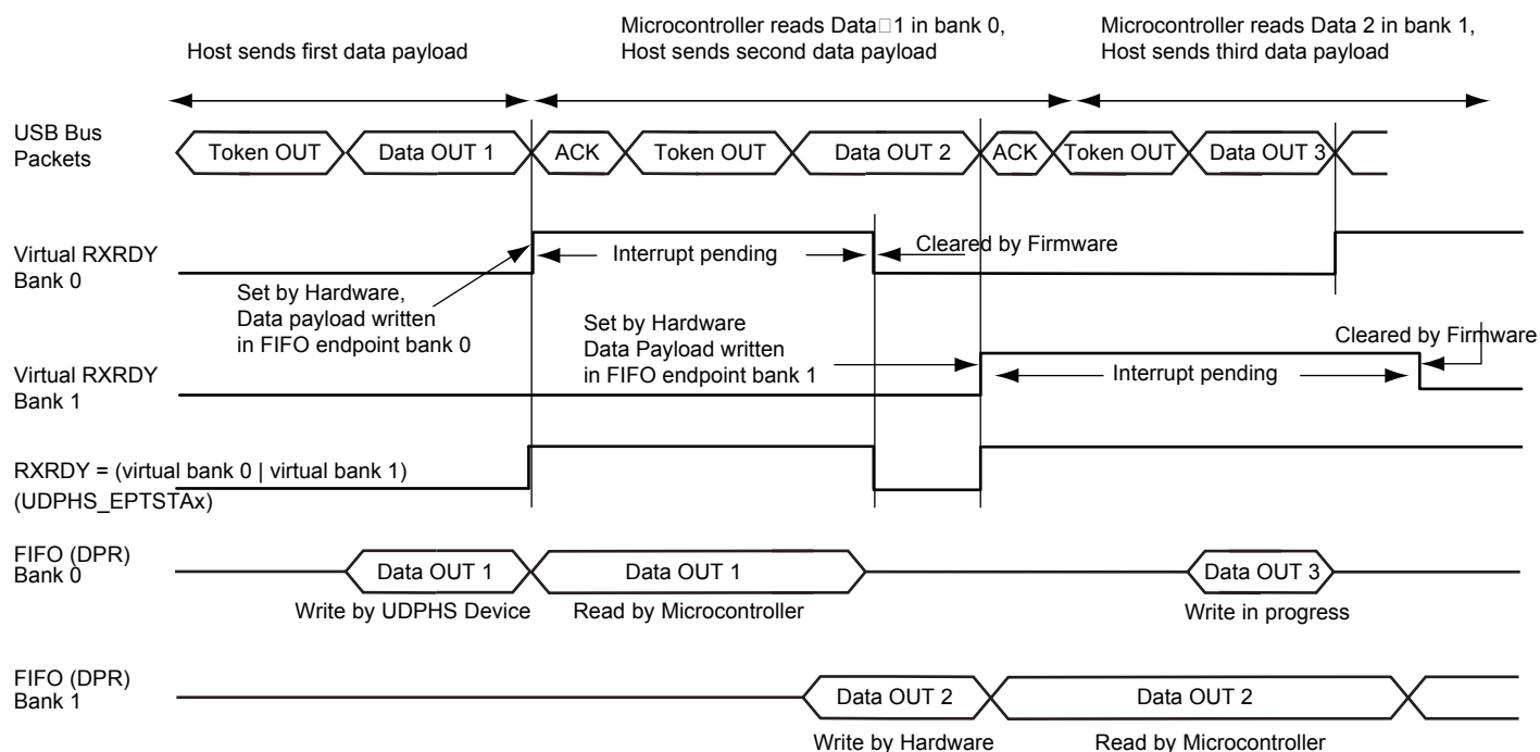
Figure 35-15. Data OUT Transfer for an Endpoint with Two Banks
