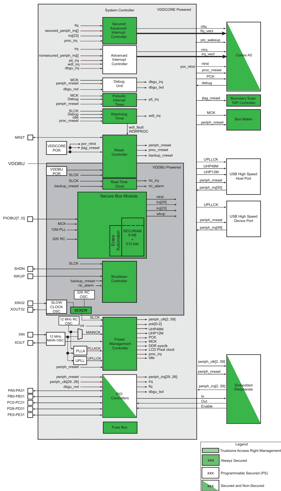
Figure 8-1. SAMA5D4 System Controller Block Diagram
