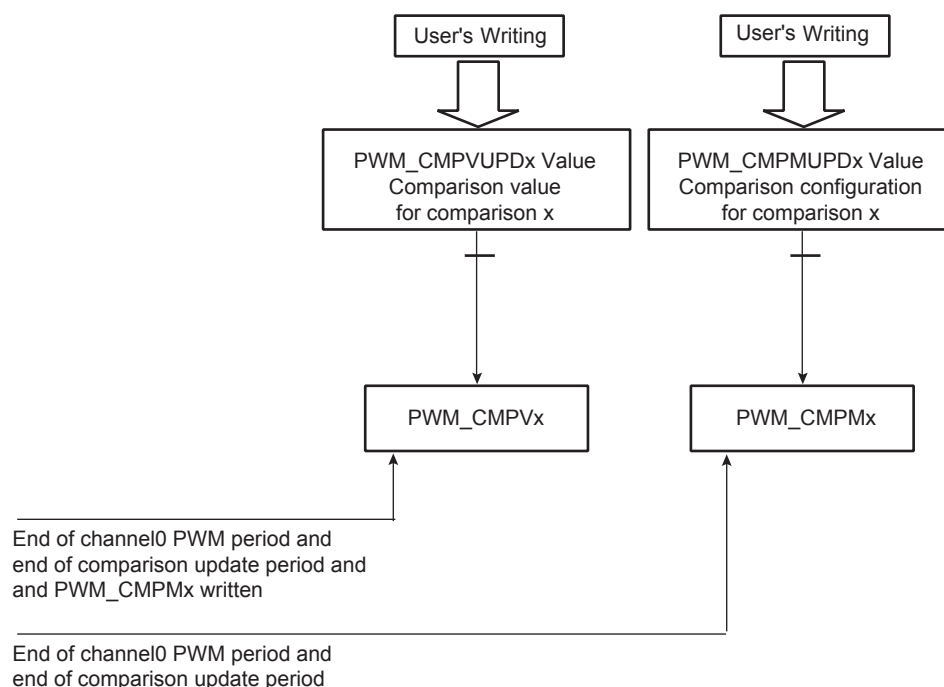
Figure 47-20. Synchronized Update of Comparison Values and Configurations
