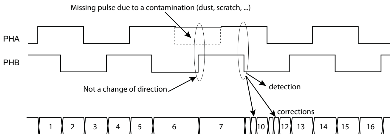
Figure 46-22. Detection and Auto-correction of Missing Pulses
