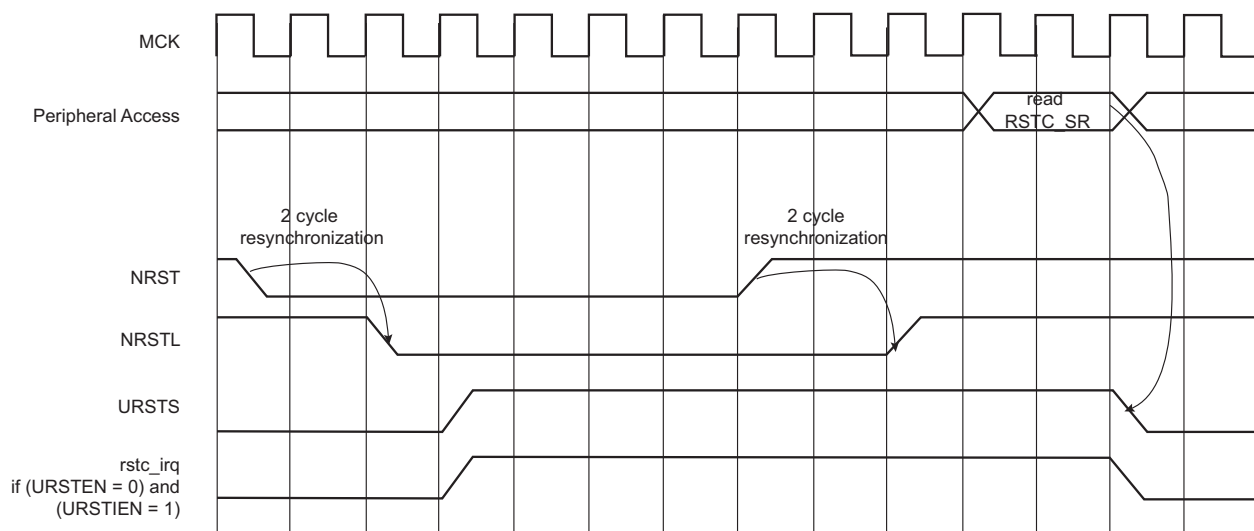
Figure 20-8. Reset Controller Status and Interrupt
