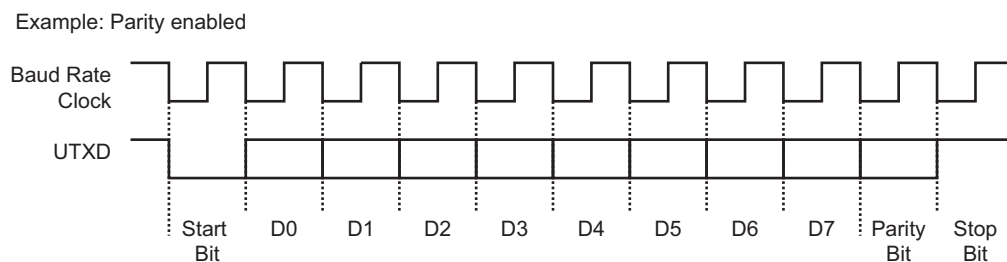
Figure 43-9. Character Transmission
