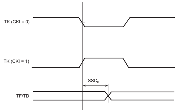
Figure 56-15. SSC Transmitter, TK and TF in Output
