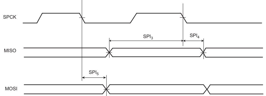
Figure 56-9. SPI Master Mode 0 and 3
