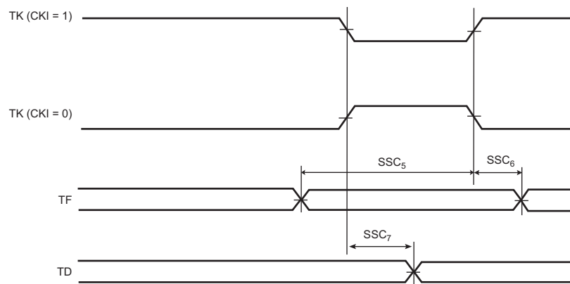
Figure 56-18. SSC Transmitter, TK and TF in Input
