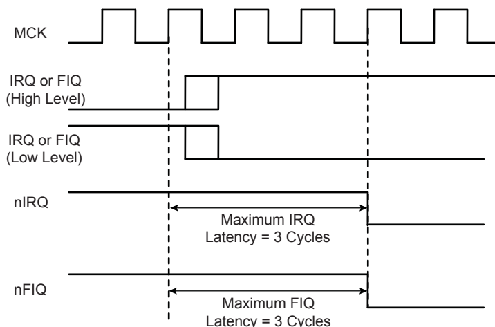
Figure 18-7. External Interrupt Level Sensitive Source
