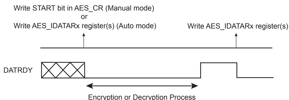
Figure 50-2. Manual and Auto Modes with AES_MR.LOD = 1
