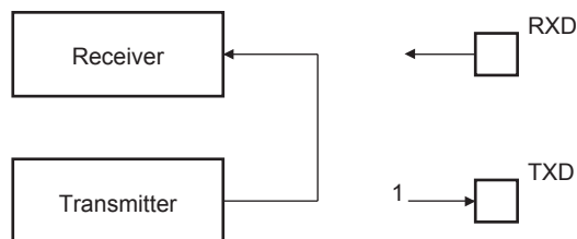
Figure 44-40. Local Loopback Mode Configuration
