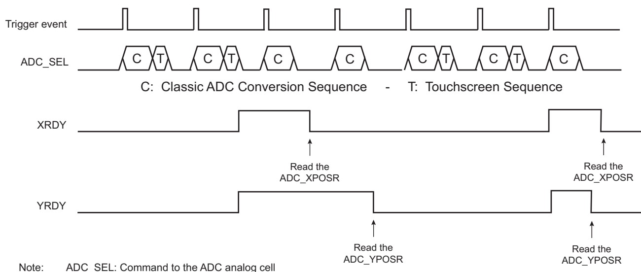
Figure 48-14. Insertion of Touchscreen Sequences (TSFREQ = 2; TSAV = 1)
