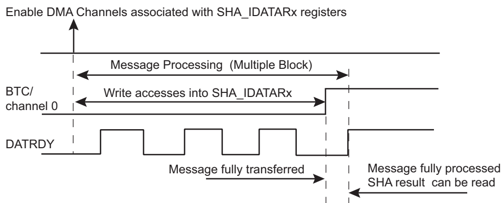
Figure 52-1. Enable DMA Channels
