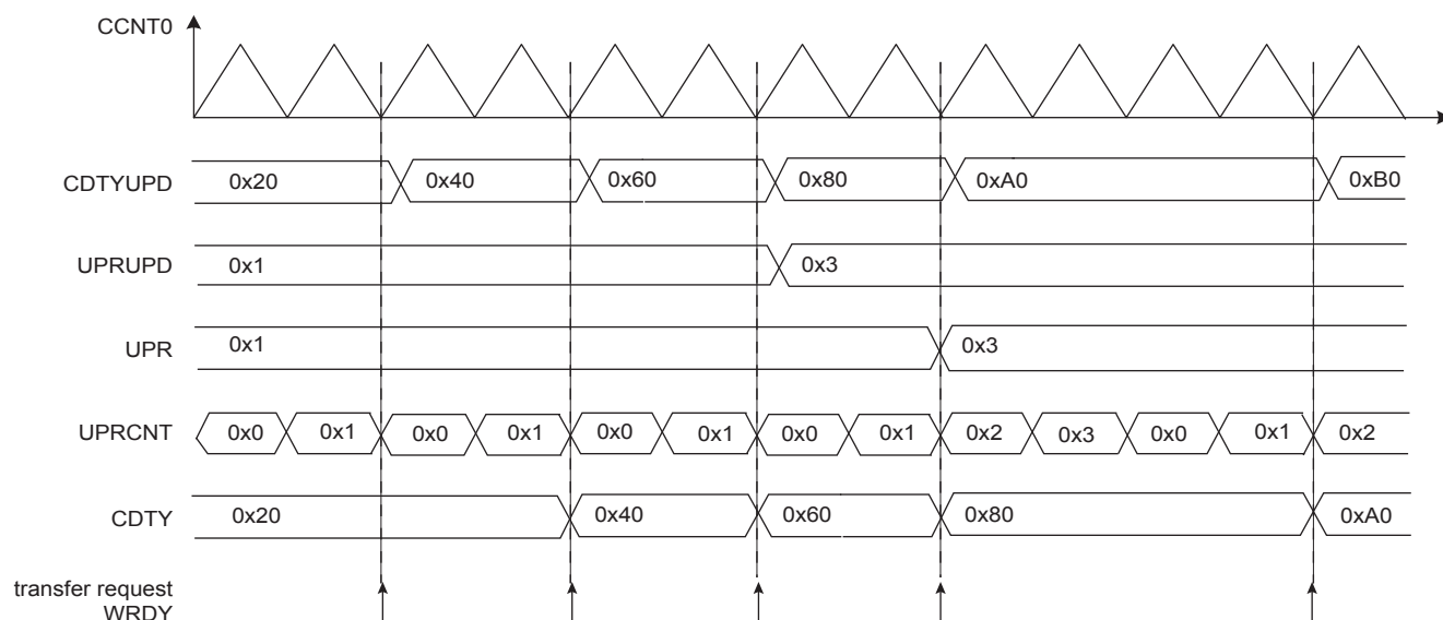
Figure 47-13. Method 3 (UPDM = 2 and PTRM = 0)
