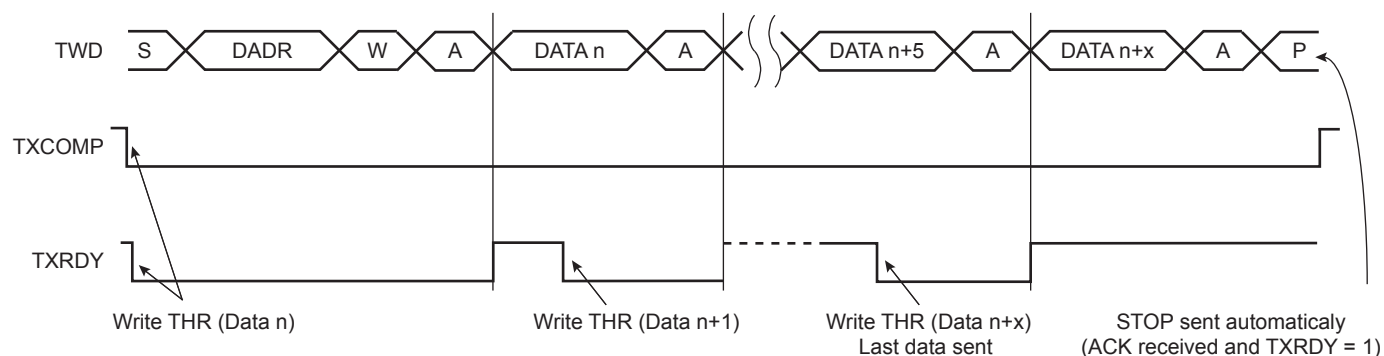
Figure 40-7. Master Write with Multiple Data Byte
