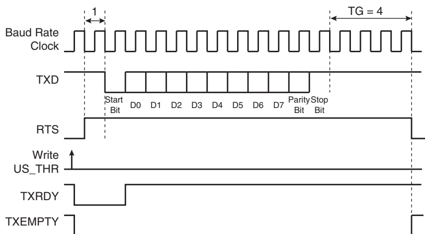
Figure 44-35. Example of RTS Drive with Timeguard
