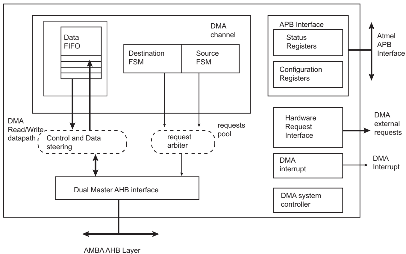
Figure 31-1. DMA Controller (XDMAC) Block Diagram
