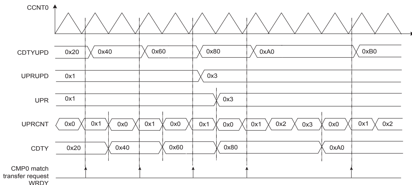
Figure 47-14. Method 3 (UPDM = 2 and PTRM = 1 and PTRCS = 0)
