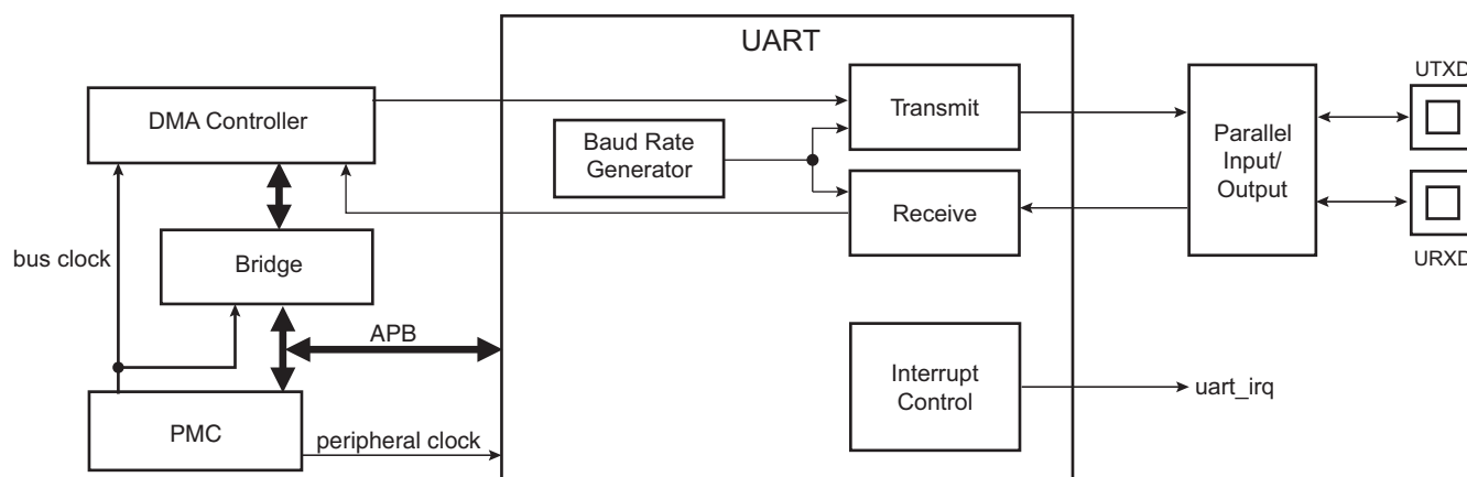
Figure 43-1. UART Functional Block Diagram
