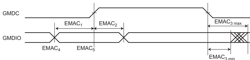
Figure 56-25. Minimum and Maximum Access Time of Ethernet MAC Output Signals
