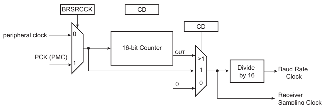
Figure 43-2. Baud Rate Generator
