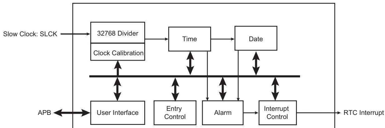
Figure 23-1. RTC Block Diagram
