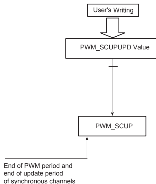
Figure 47-19. Synchronized Update of Update Period Value of Synchronous Channels
