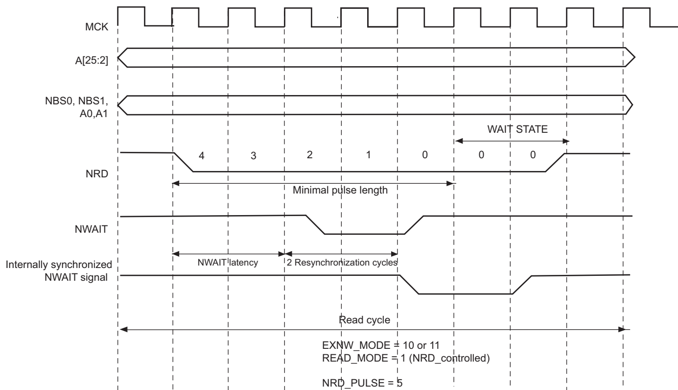
Figure 30-27. NWAIT Latency
