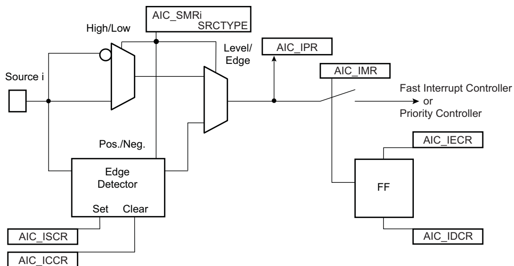
Figure 18-5. External Interrupt Source Input Stage
