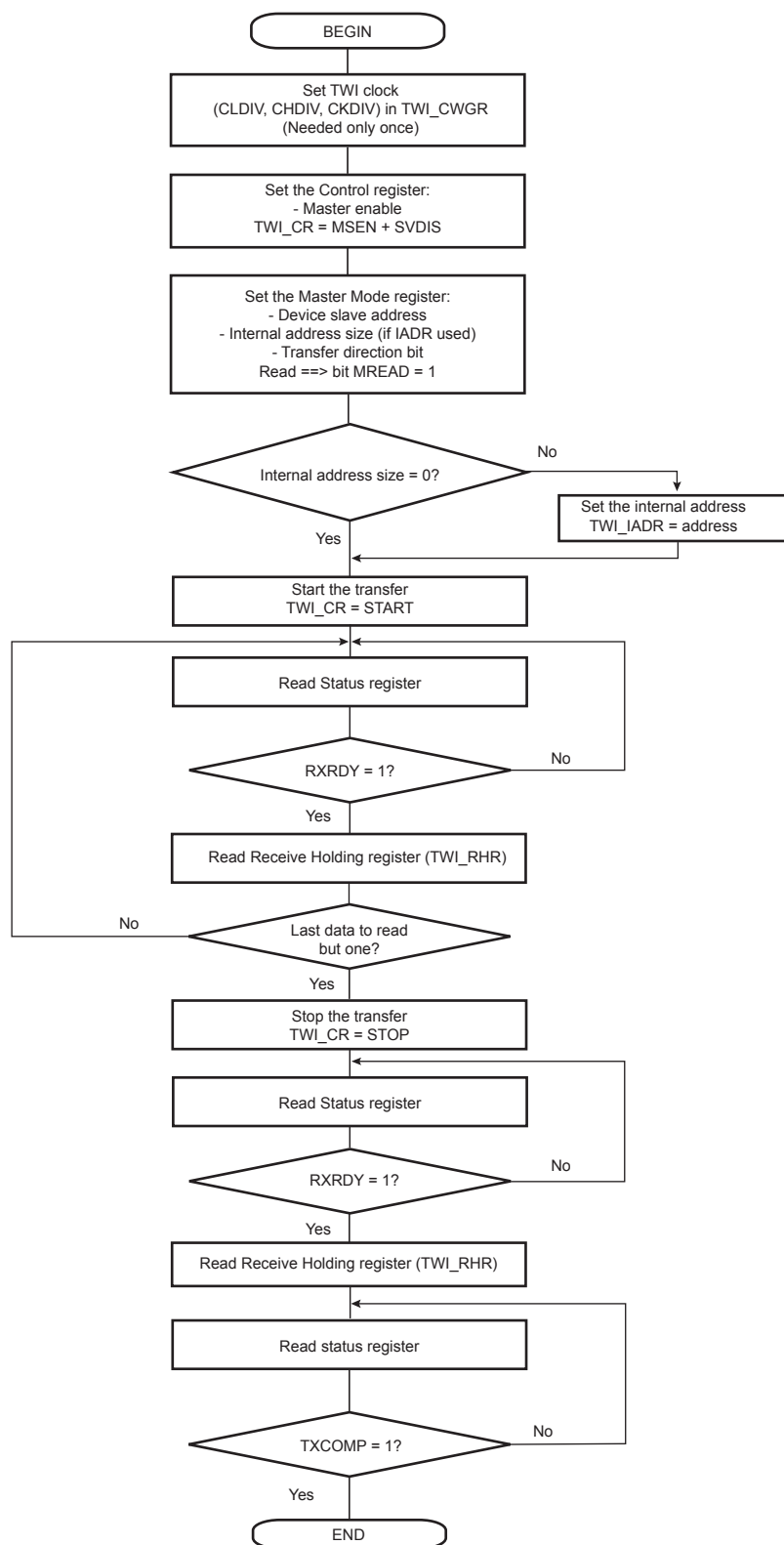
Figure 40-20. TWI Read Operation with Multiple Data Bytes with or without Internal Address
