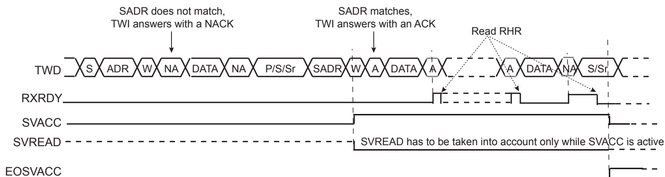
Figure 40-26. Write Access Ordered by a Master
