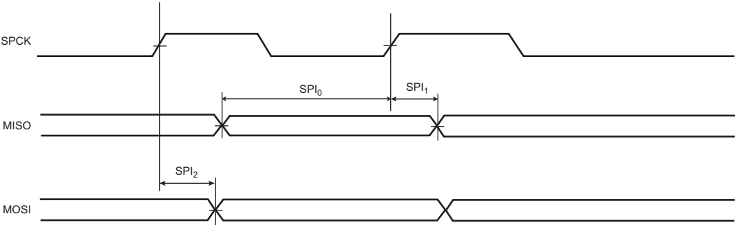
Figure 56-8. SPI Master Mode 1 and 2
