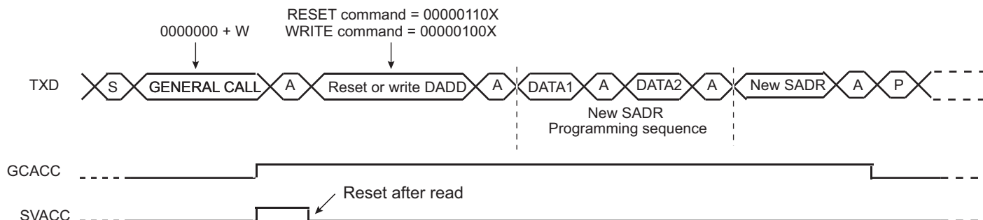
Figure 40-27. Master Performs a General Call
