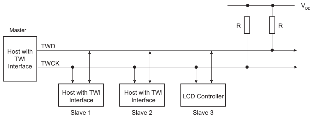
Figure 40-24. Slave Mode Typical Application Block Diagram
