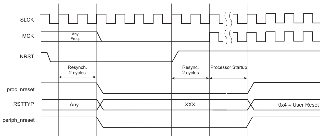
Figure 20-5. User Reset State
