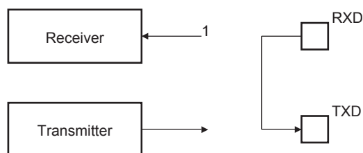
Figure 44-41. Remote Loopback Mode Configuration
