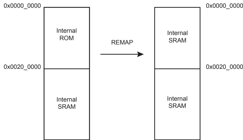
Figure 13-4. Remap Action after Download Completion
