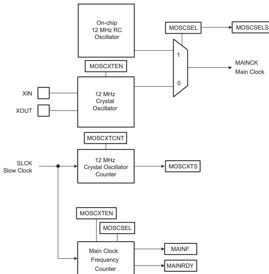
Figure 26-3. Main Clock Block Diagram
