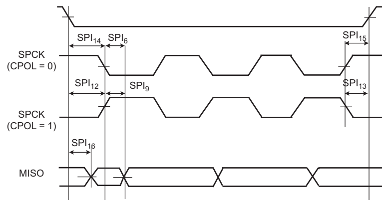
Figure 56-12. SPI Slave Mode - NPCS Timings
