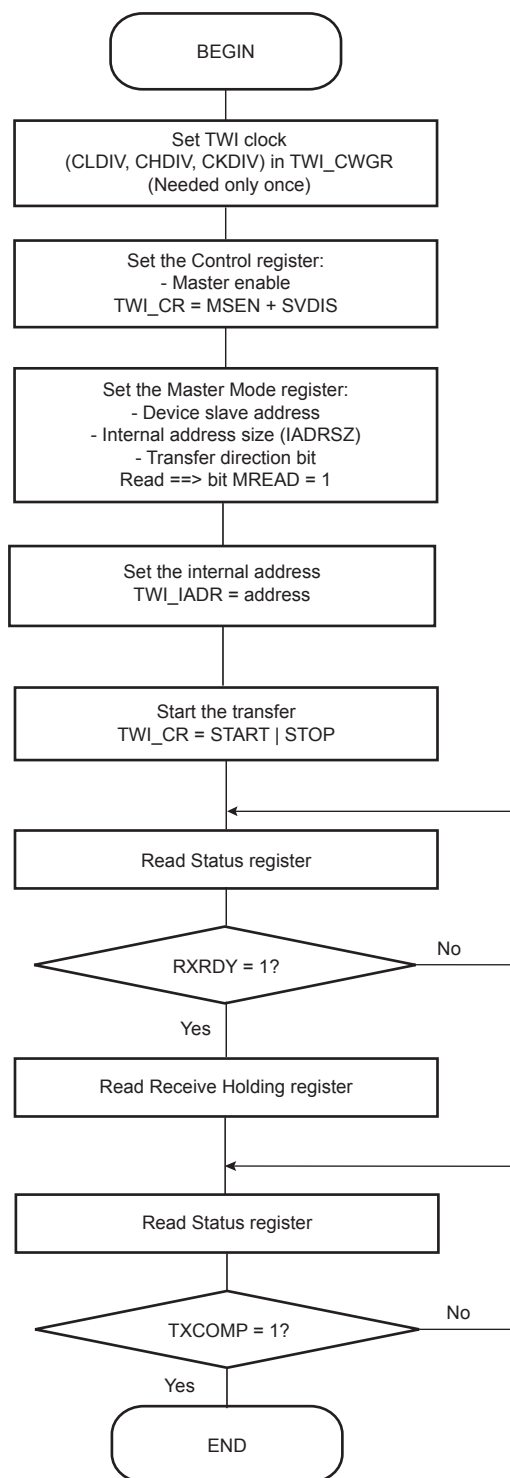
Figure 40-19. TWI Read Operation with Single Data Byte and Internal Address
