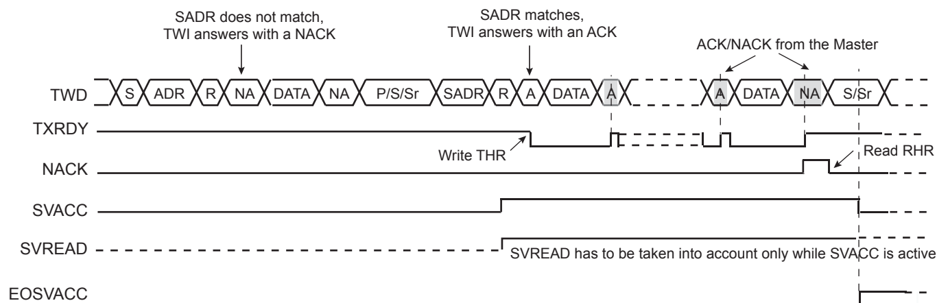
Figure 40-25. Read Access Ordered by a MASTER
