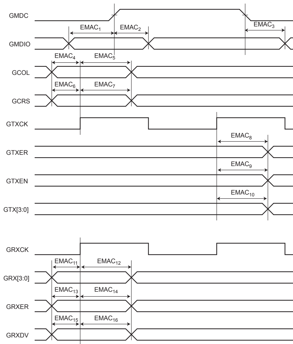
Figure 56-26. Ethernet MAC MII Mode
