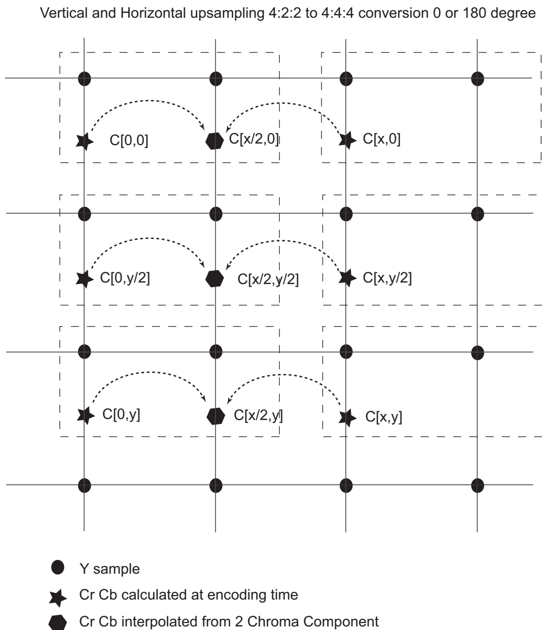
Figure 32-2. 4:2:2 Upsampling Algorithm
