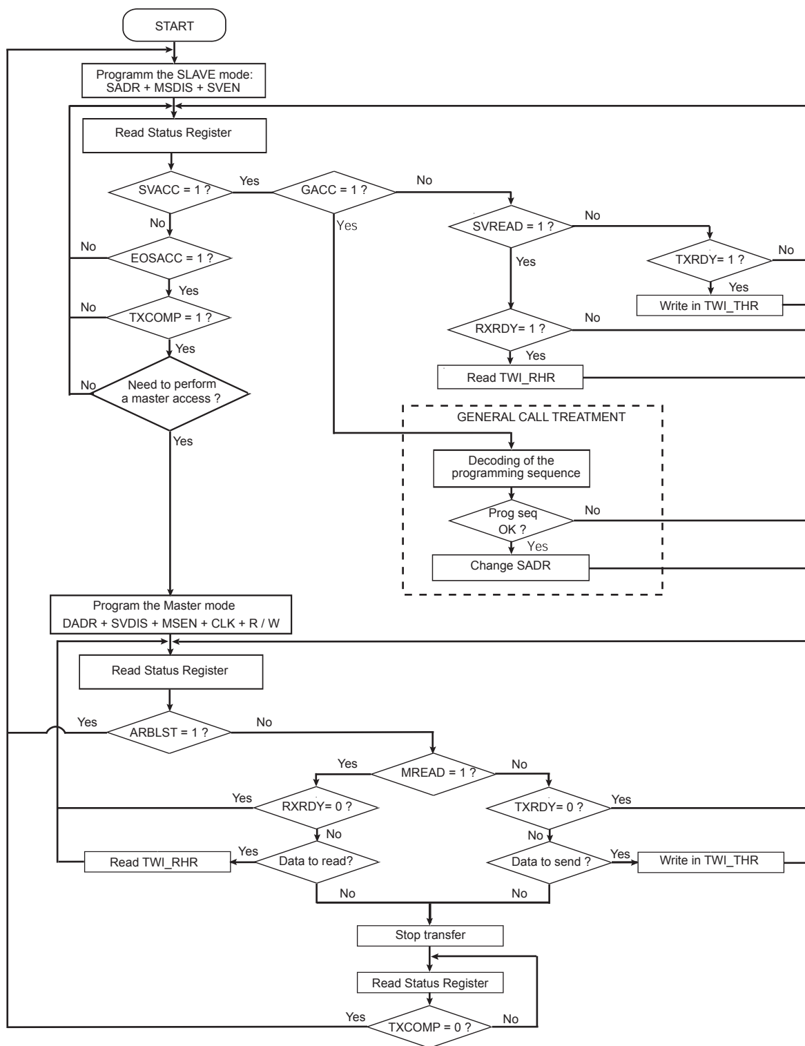
Figure 40-23. Multi-master Flowchart
