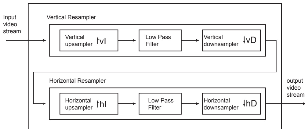
Figure 32-6. Video Resampler Architecture
