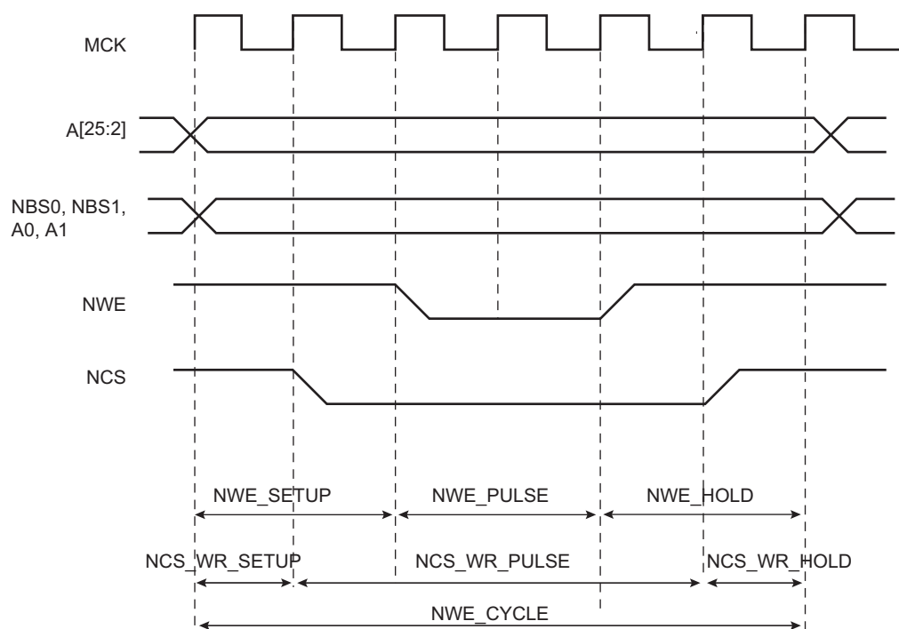
Figure 30-10. Write Cycle
