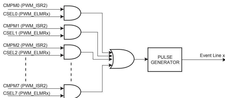
Figure 47-17. Event Line Block Diagram
