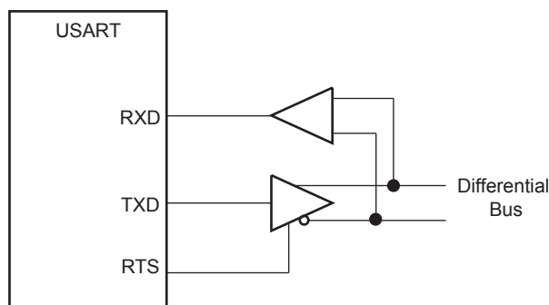
Figure 44-34. Typical Connection to a RS485 Bus
