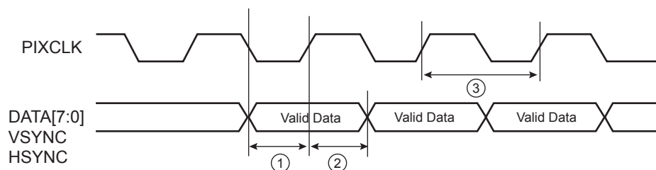
Figure 56-24. ISI Timing Diagram
