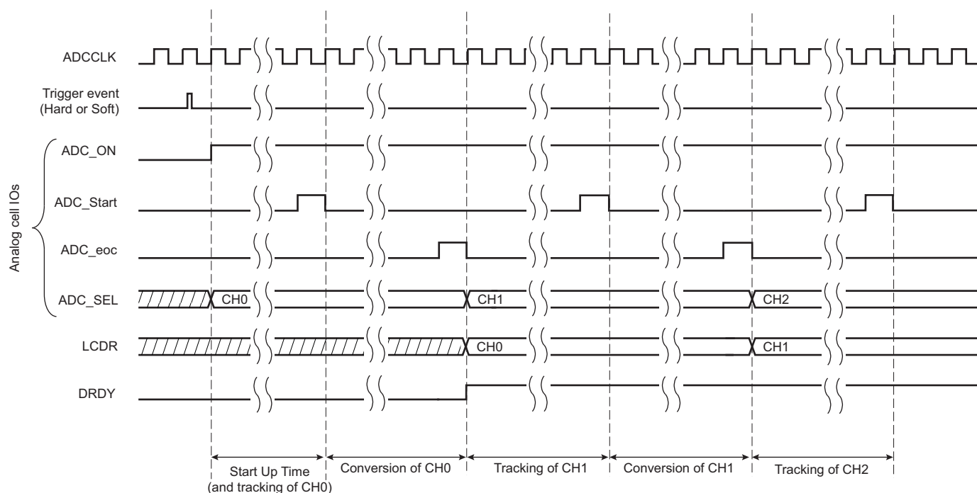
Figure 48-2. Sequence of ADC Conversions
