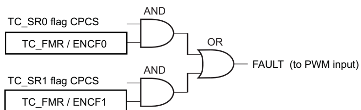
Figure 46-24. Fault Output Generation
