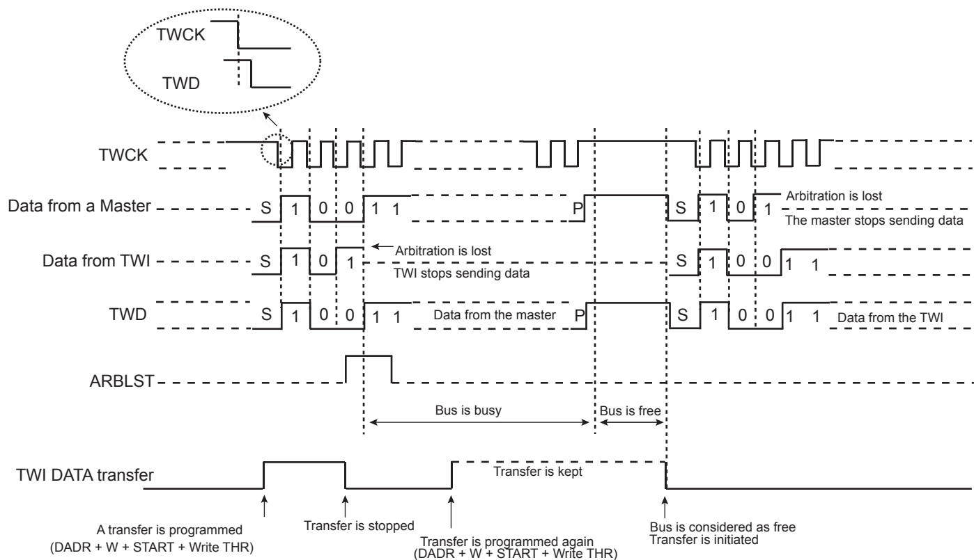
Figure 40-22. Arbitration Cases
