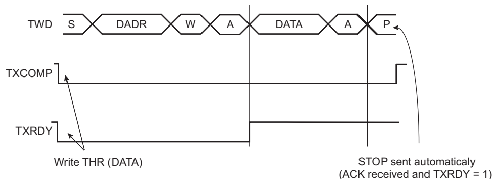
Figure 40-6. Master Write with One Data Byte
