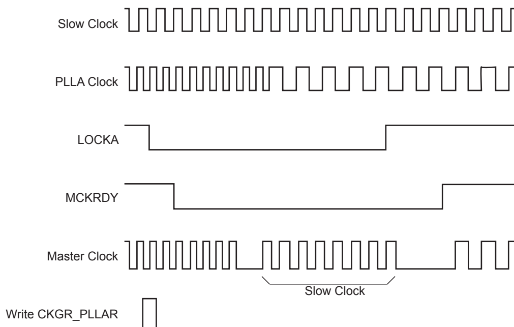
Figure 27-7. Change PLLA Programming
