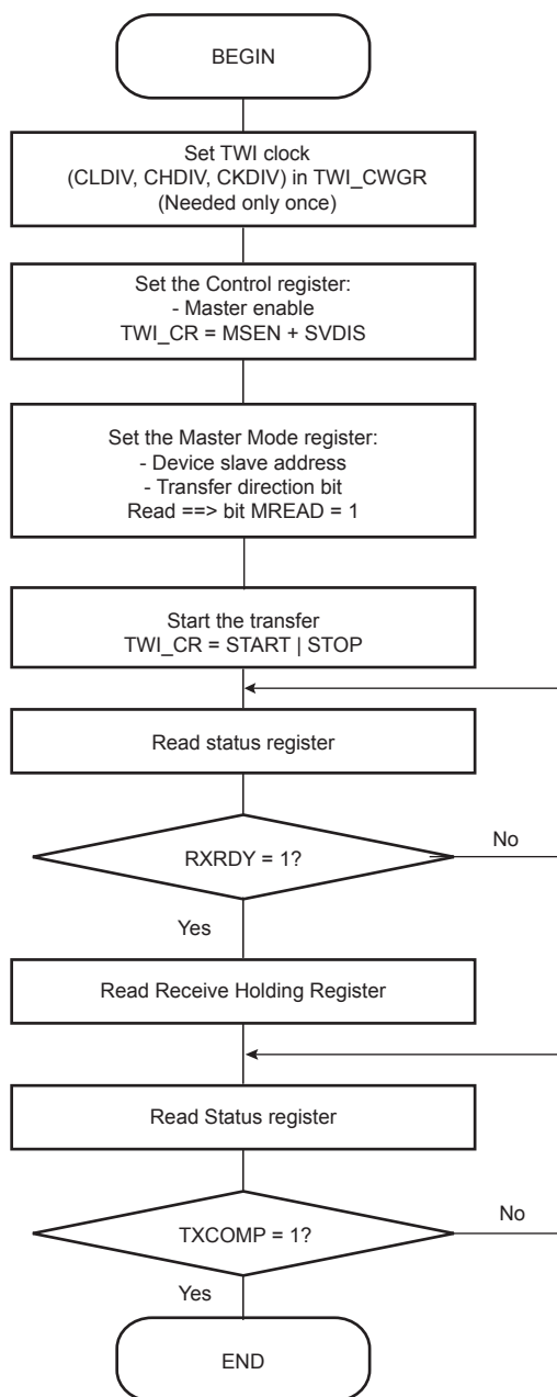
Figure 40-18. TWI Read Operation with Single Data Byte without Internal Address
