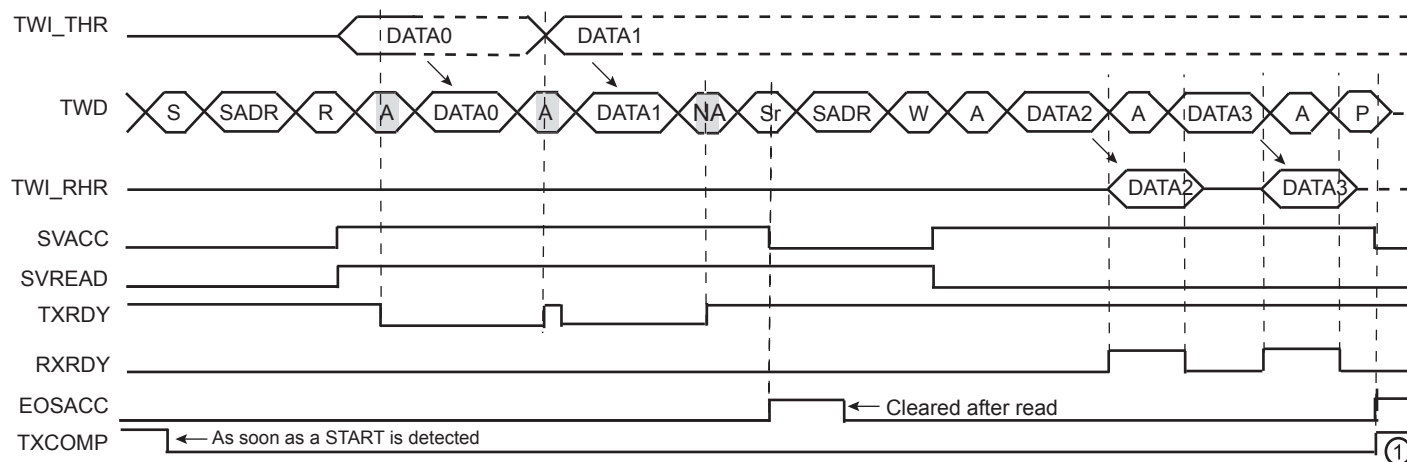
Figure 40-30. Repeated Start + Reversal from Read to Write Mode
