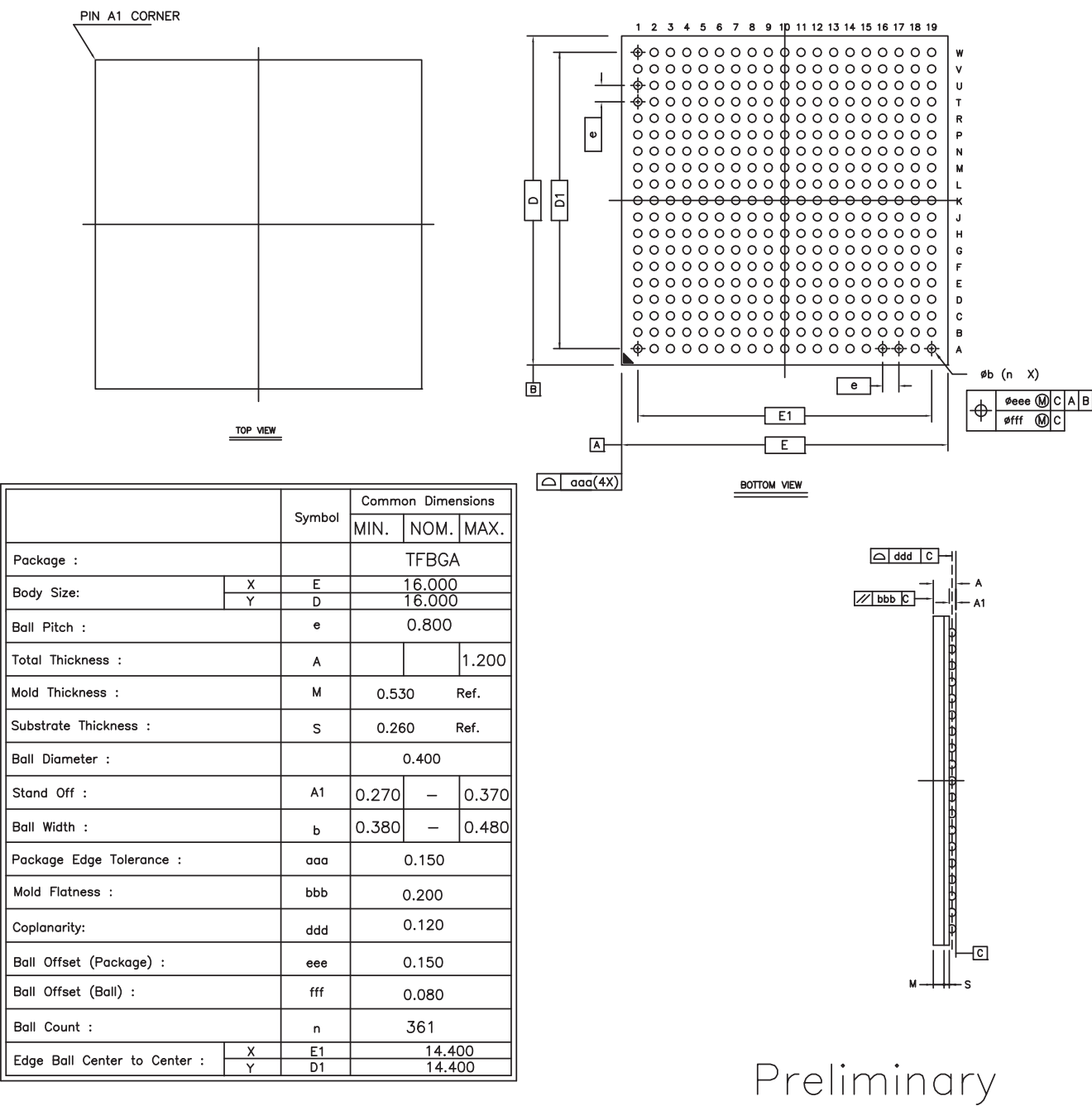
Figure 57-1. 361-ball LFBGA Package Drawing
