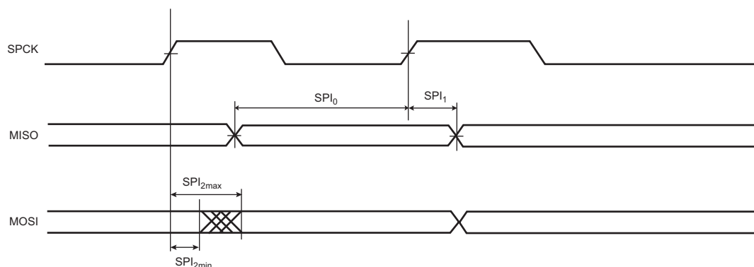
Figure 56-13. Minimum and Maximum Access Time for SPI Output Signal
