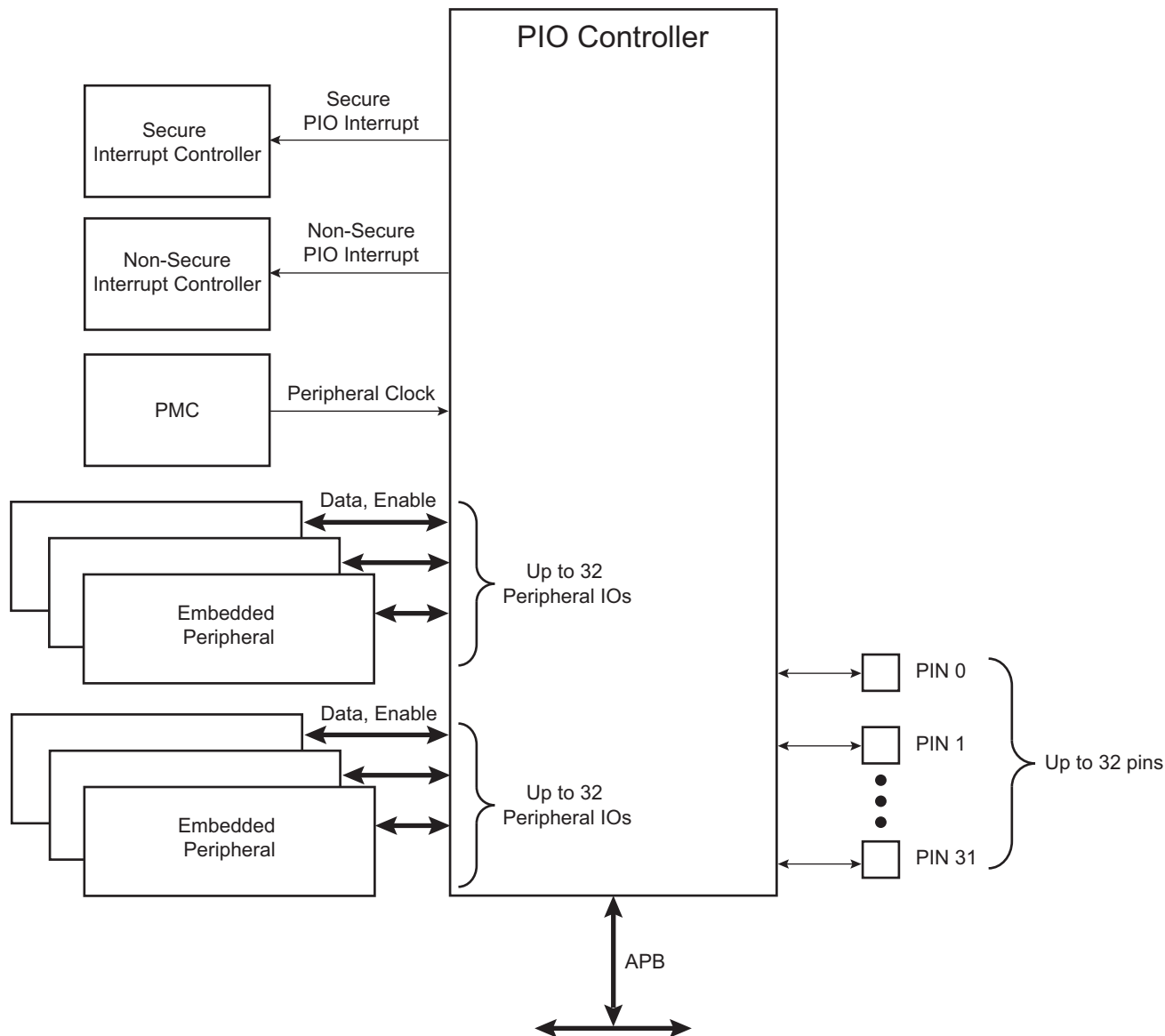
Figure 28-1. Block Diagram
