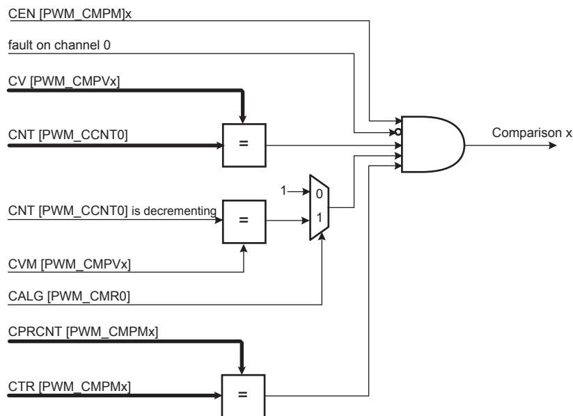
Figure 47-15. Comparison Unit Block Diagram
