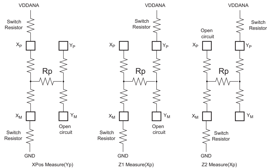
Figure 48-11. Pressure Measurement
