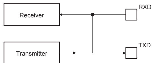
Figure 44-39. Automatic Echo Mode Configuration
