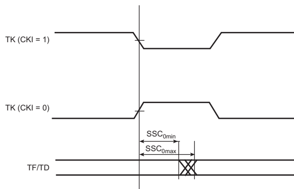
Figure 56-23. Minimum and Maximum Access Time of Output Signals
