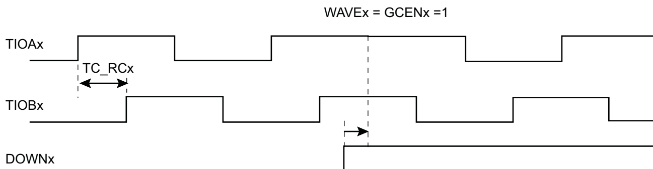
Figure 46-23. 2-bit Gray Up/Down Counter
