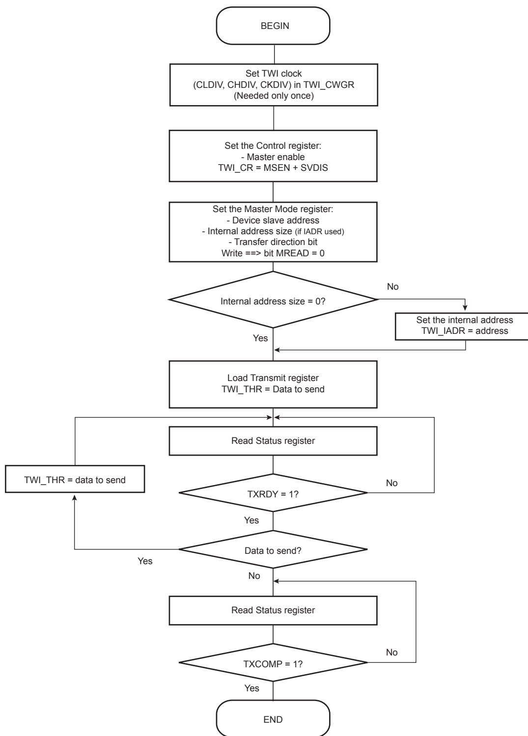
Figure 40-17. TWI Write Operation with Multiple Data Bytes with or without Internal Address
