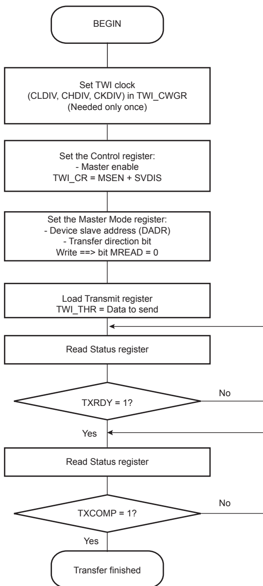
Figure 40-15. TWI Write Operation with Single Data Byte without Internal Address
