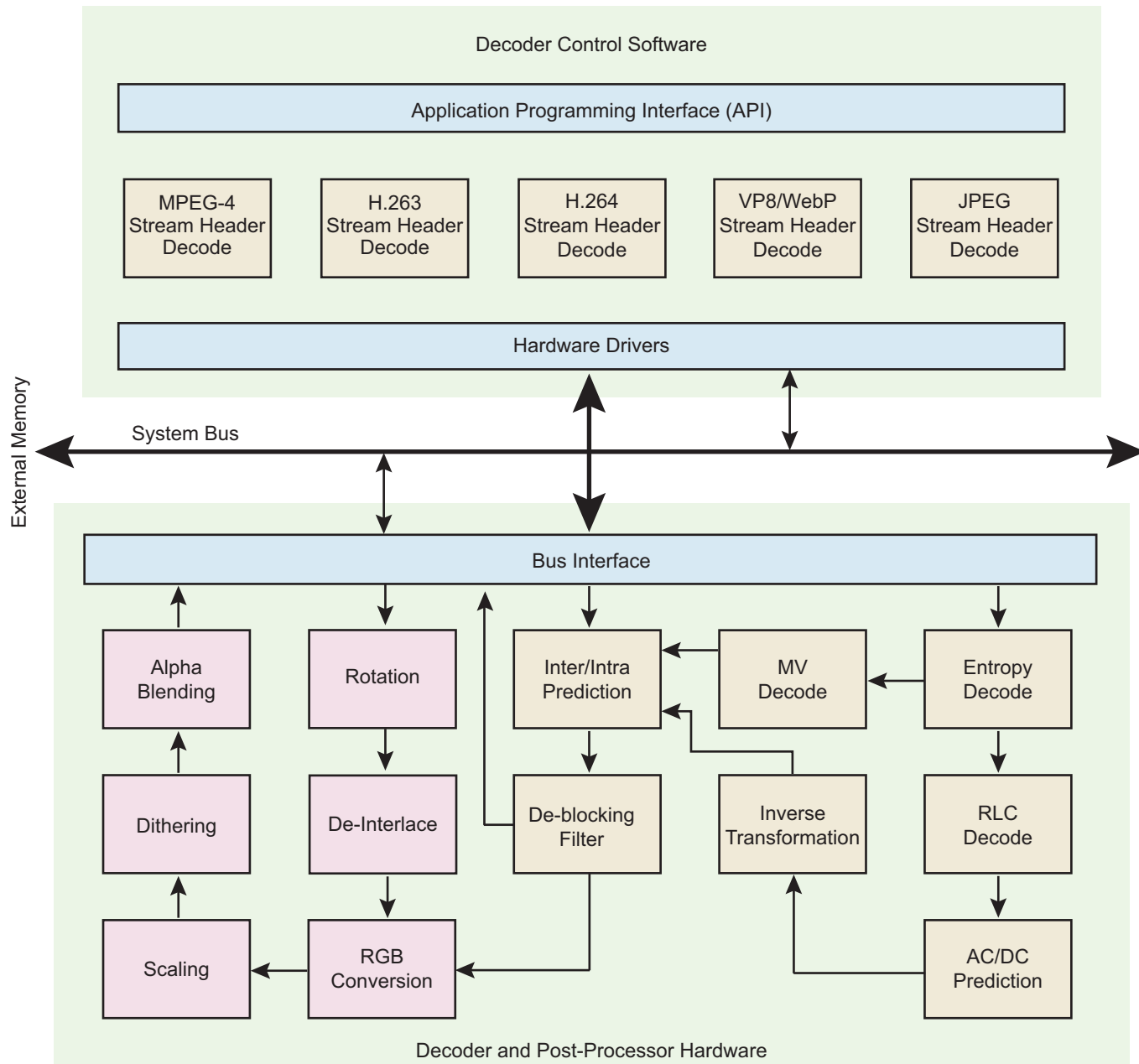
Figure 33-1. Block Diagram
