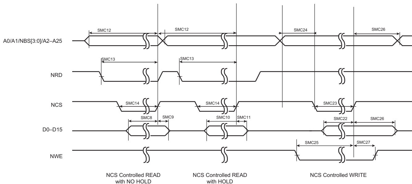
Figure 56-6. SMC Timings - NCS Controlled Read and Write
