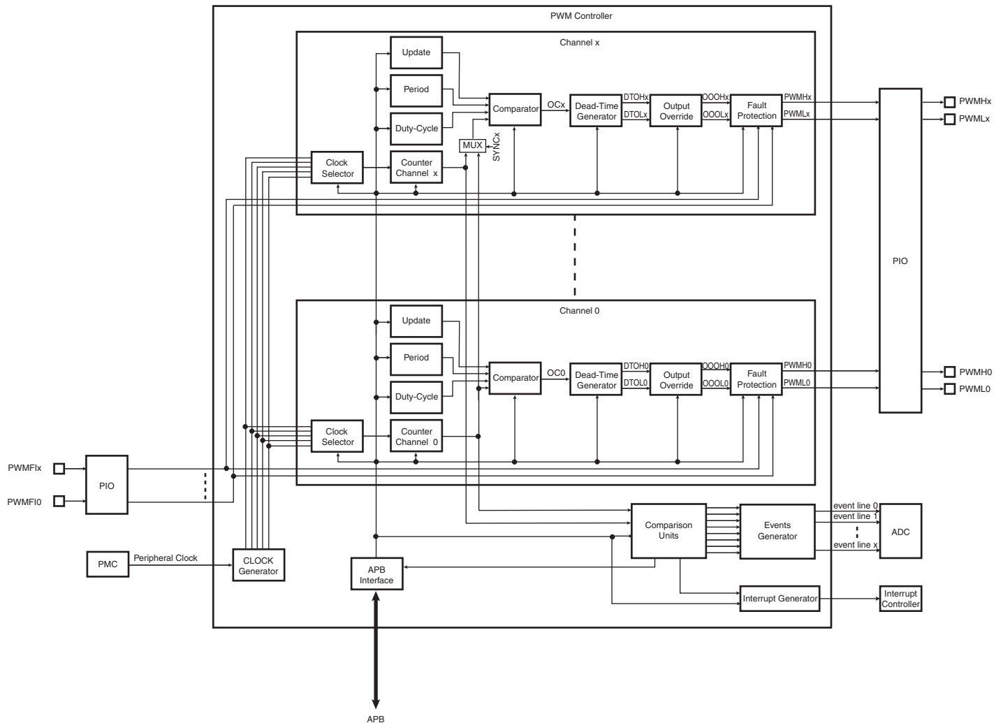
Figure 47-1. Pulse Width Modulation Controller Block Diagram
