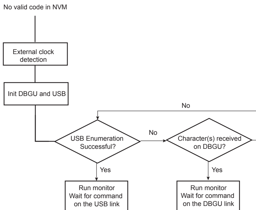
Figure 13-10. SAM-BA Monitor Diagram
