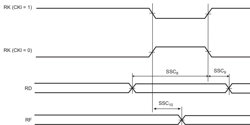
Figure 56-20. SSC Receiver, RK in Input and RF in Output
