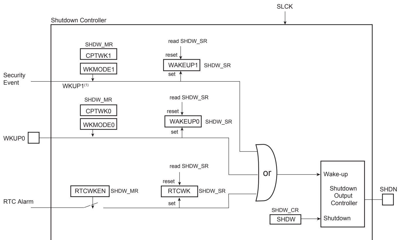
Figure 21-1. Shutdown Controller Block Diagram
