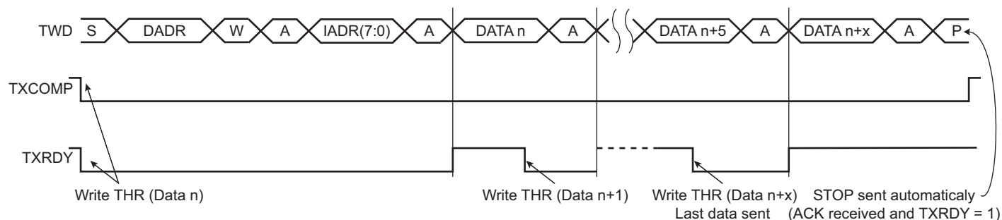
Figure 40-8. Master Write with One Byte Internal Address and Multiple Data Bytes
