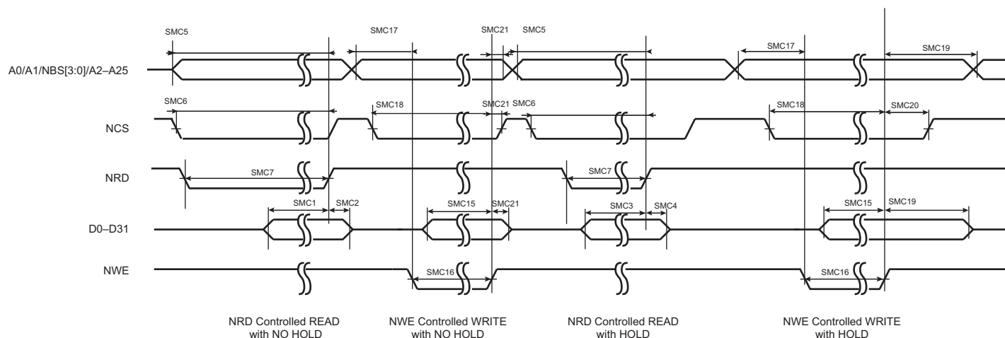
Figure 56-7. SMC Timings - NRD Controlled Read and NWE Controlled Write
