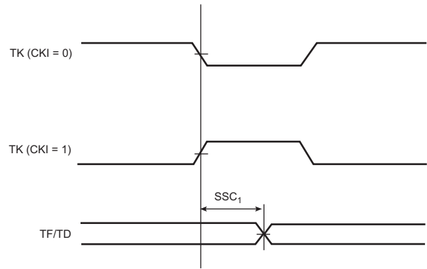
Figure 56-16. SSC Transmitter, TK in Input and TF in Output
