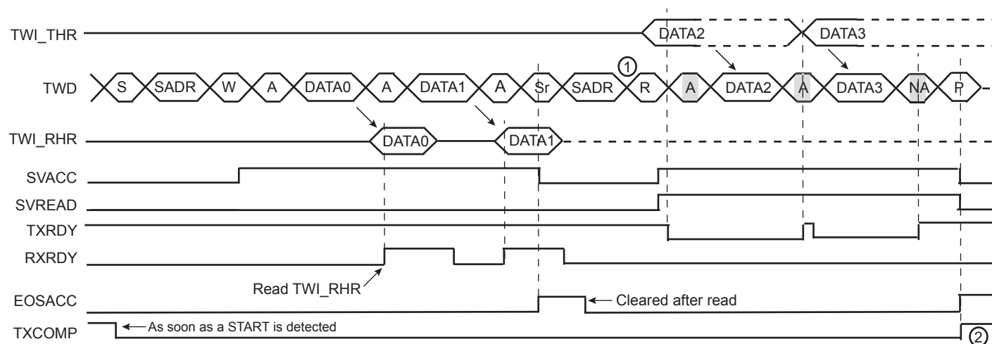
Figure 40-31. Repeated Start + Reversal from Write to Read Mode
