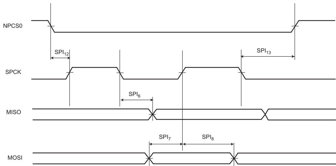
Figure 56-10. SPI Slave Mode 0 and 3
