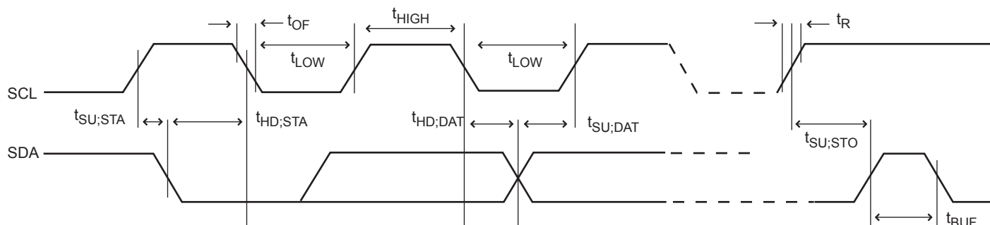
Figure 56-31. Two-wire Serial Bus Timing
