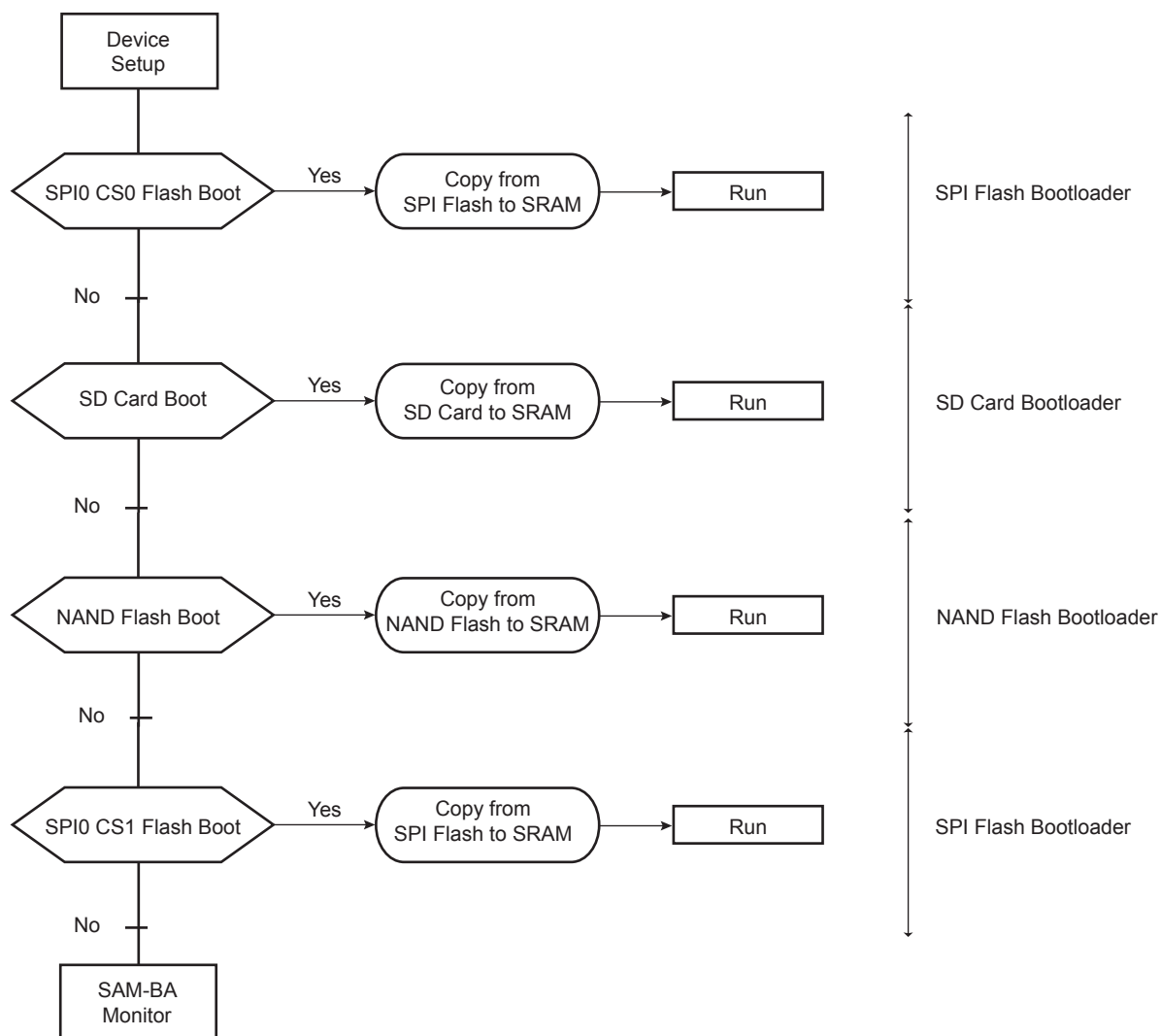
Figure 13-2. NVM Bootloader Sequence Diagram
