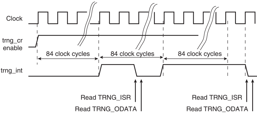
Figure 49-2. TRNG Data Generation Sequence
