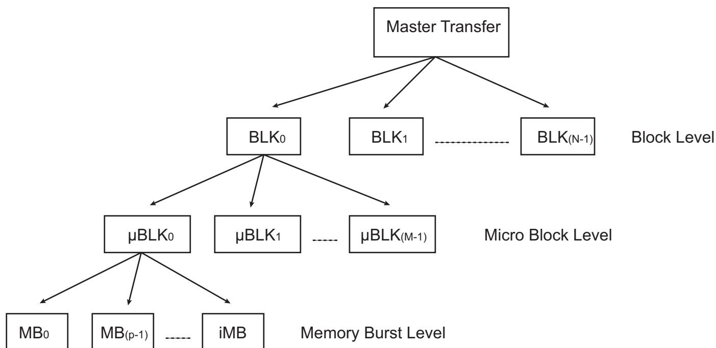
Figure 31-2. XDAMC Memory Transfer Hierarchy
