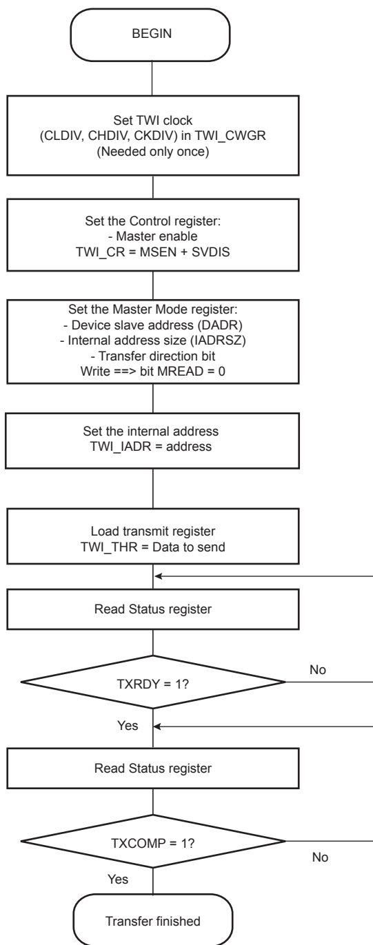
Figure 40-16. TWI Write Operation with Single Data Byte and Internal Address
