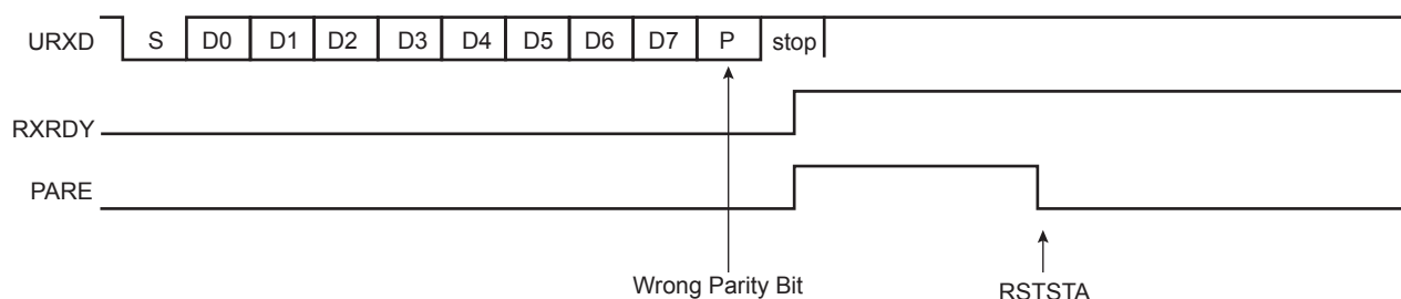
Figure 43-7. Parity Error
