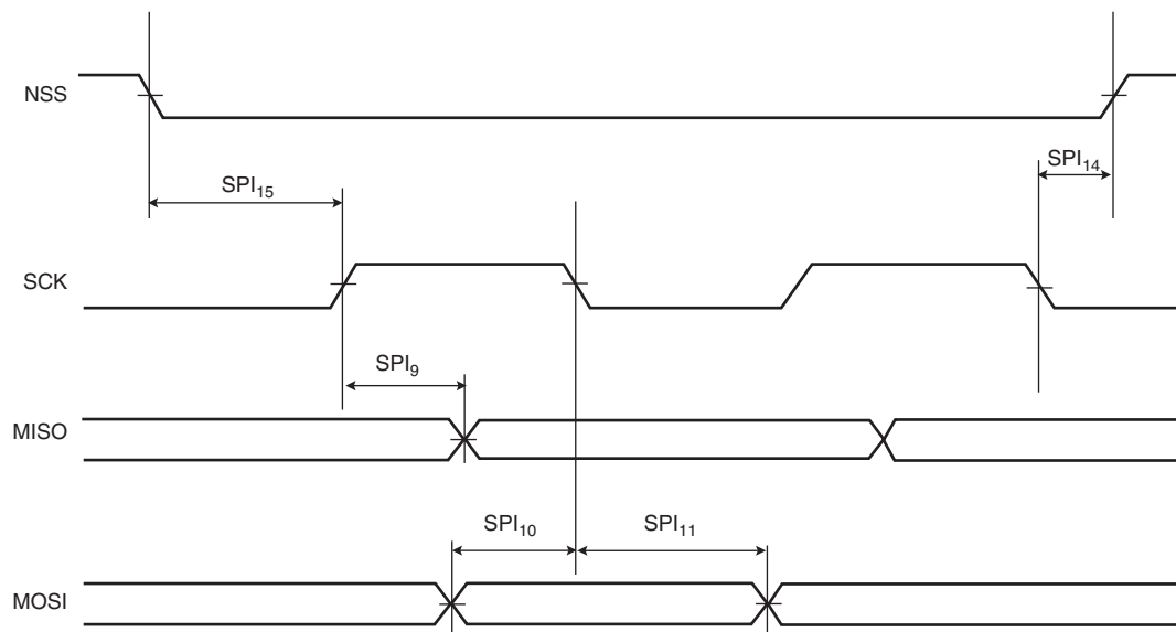
Figure 56-30. USART SPI Slave Mode 0 or 3
