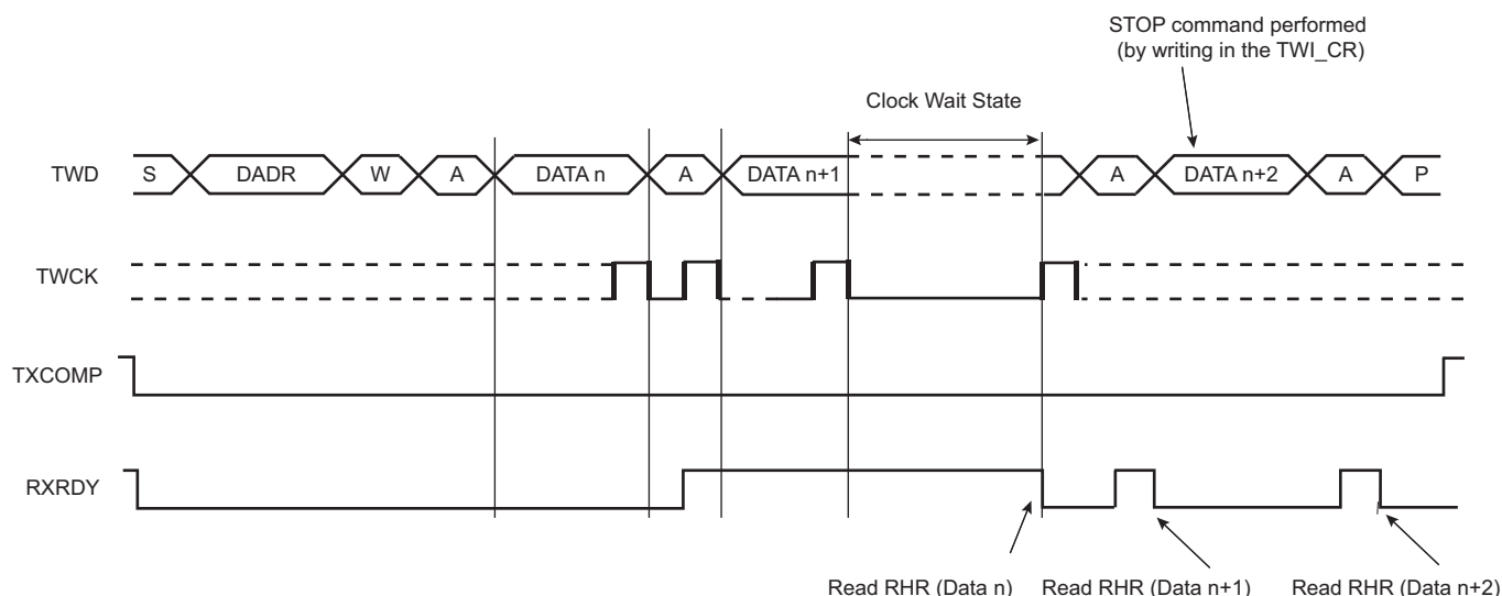
Figure 40-11. Master Read Wait State with Multiple Data Bytes
