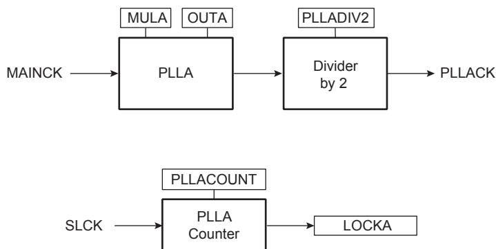
Figure 26-4. Divider and PLLA Block Diagram
