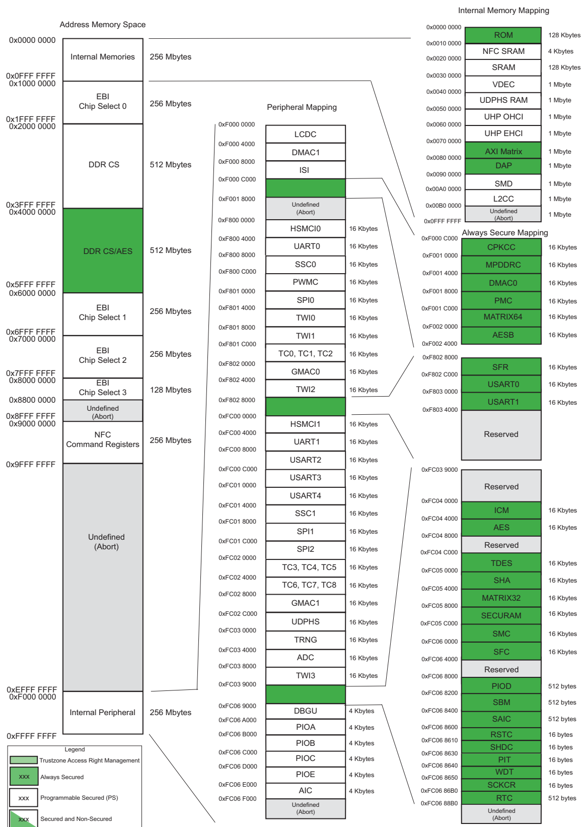
Figure 6-1. SAMA5D4 Series Memory Mapping
