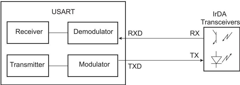
Figure 44-31. Connection to IrDA Transceivers
