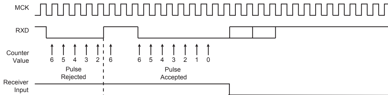
Figure 44-33. IrDA Demodulator Operations
