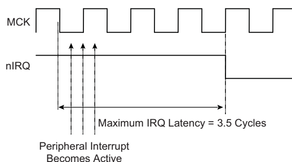
Figure 18-9. Internal Interrupt Level Sensitive Source
