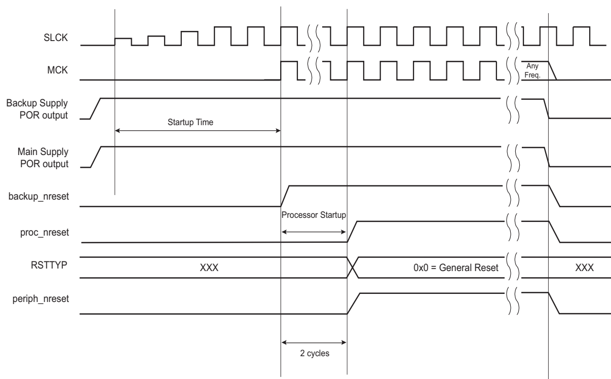
Figure 20-3. General Reset State
