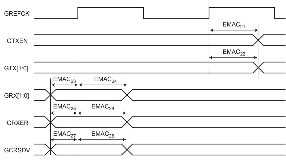
Figure 56-27. Ethernet MAC RMII Timings
