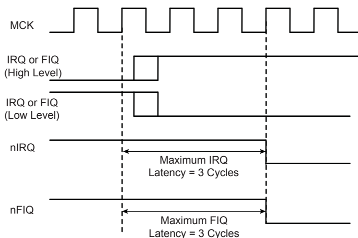
Figure 18-8. Internal Interrupt Edge Triggered Source
