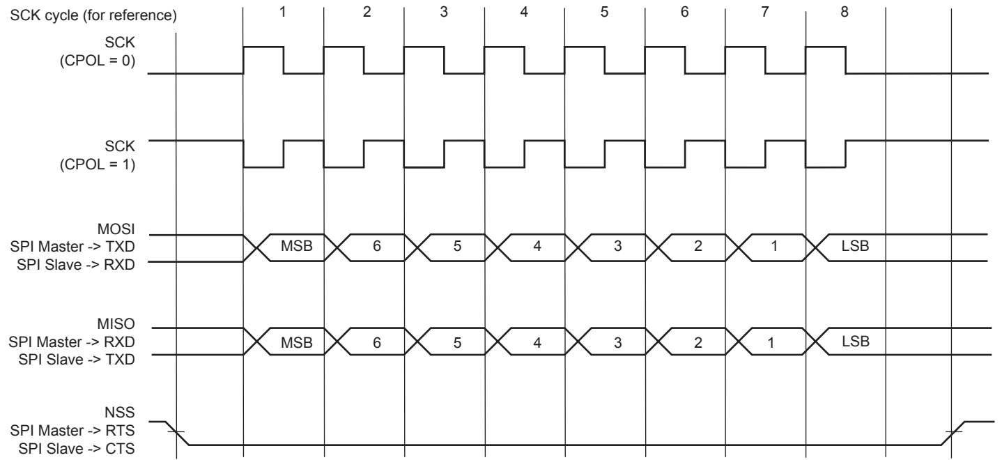
Figure 44-37. SPI Transfer Format (CPHA = 0, 8 bits per transfer)
