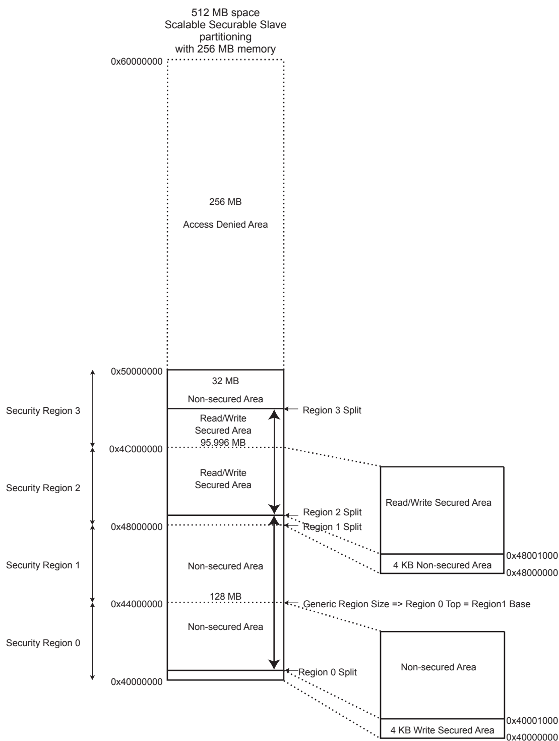
Figure 16-4. Partitioning example of a Scalable Securable slave featuring 4 equally sized security regions of 1 MB to 128 MB each and up to 8 security areas of 4 KB to 128 MB
