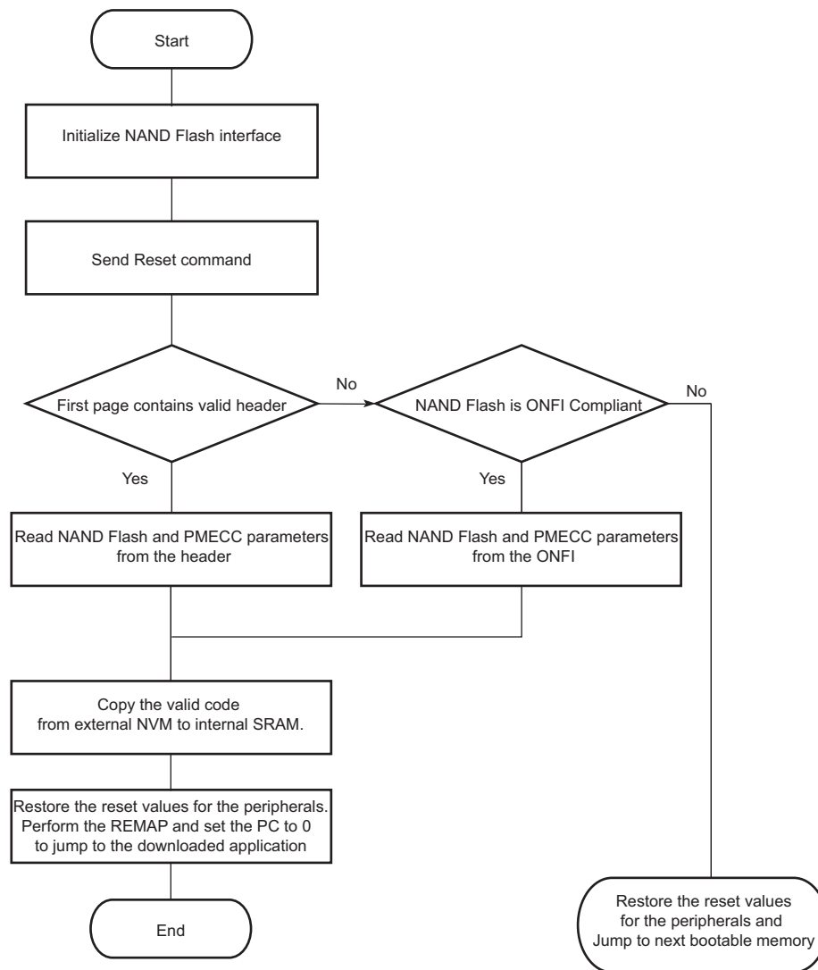
Figure 13-8. Boot NAND Flash Download
