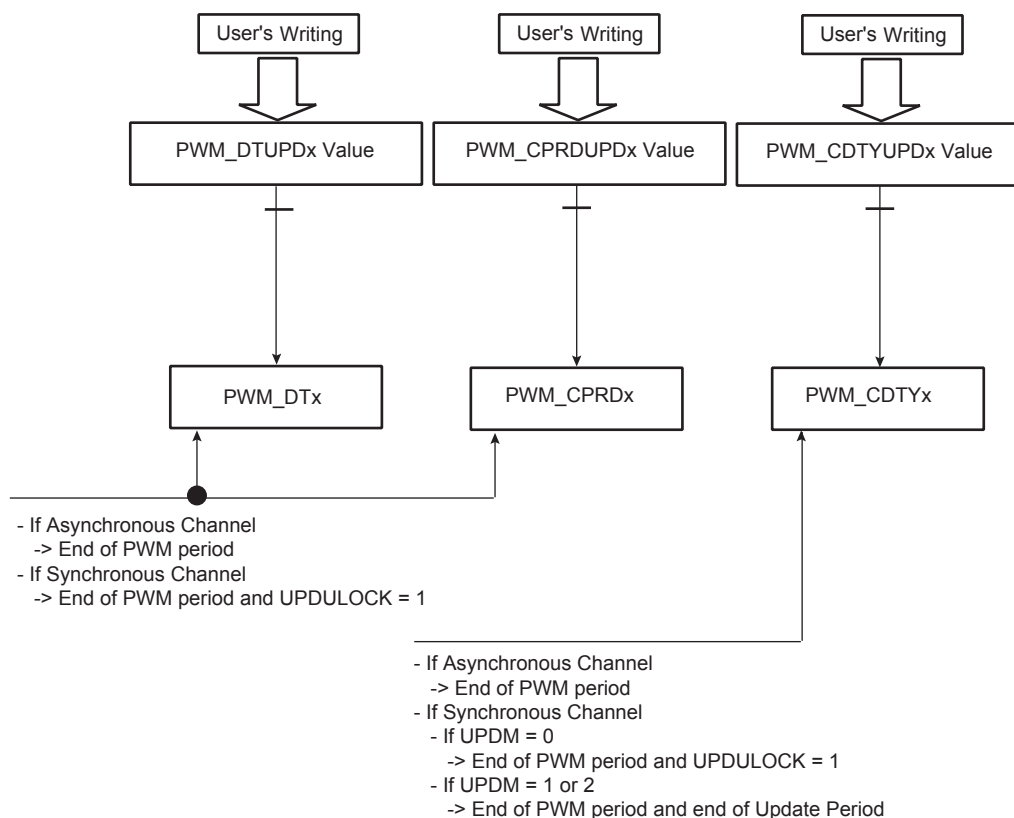
Figure 47-18. Synchronized Period, Duty-Cycle and Dead-Time Update
