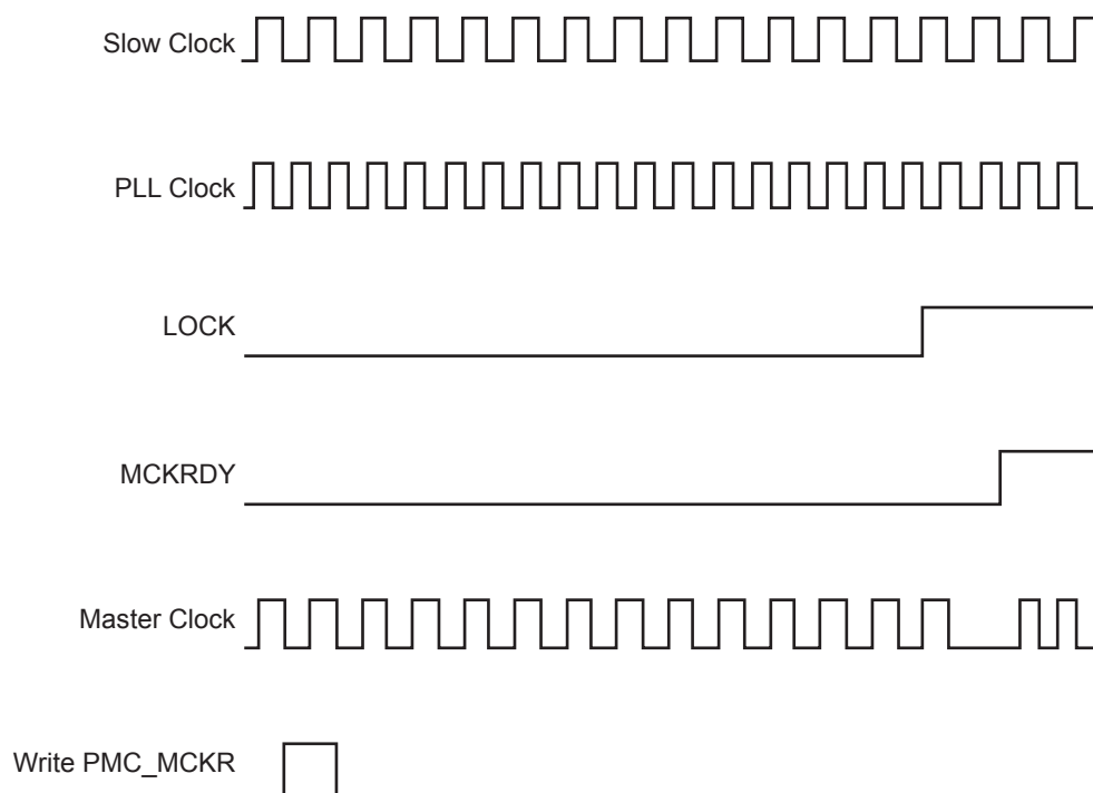
Figure 27-5. Switch Master Clock from Slow Clock to PLL Clock
