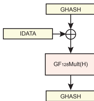
Figure 50-7. Single GHASH H Block Diagram (AADLEN ≤ 0x10 and CLEN = 0)
