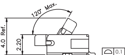
ACCOMODATED FFC/FPC
