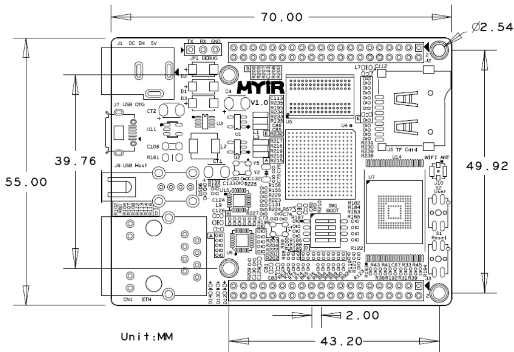
Figure 1-9 Dimension Chart of MYS-6ULX Single Board Computer
