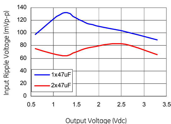
Figure 34. Input ripple voltage for various output voltages with 1x47 µF or 2x47 µF ceramic capacitors at the input (12A load). Input voltage is 5V.
