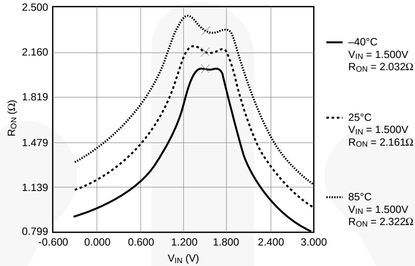
Figure 6. R_{\text{ON}} Switch On Resistance, I_{\text{ON}} = 100\text{mA} , V_{\text{CC}} = 2.7
