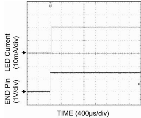
Figure 10. PWM Signal at 100% Duty Cycle ( I_{avg} = 20mA )
