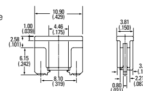
Low Profile MINI dimensions in mm (inches)
