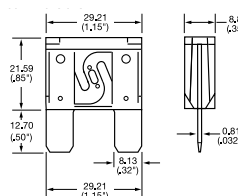
MAXI dimensions in mm (inches)
