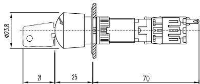
15 emergency stop switch 55 - 70 mm page 594
