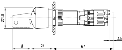
14 emergency stop switch 55 - 70 mm page 594
