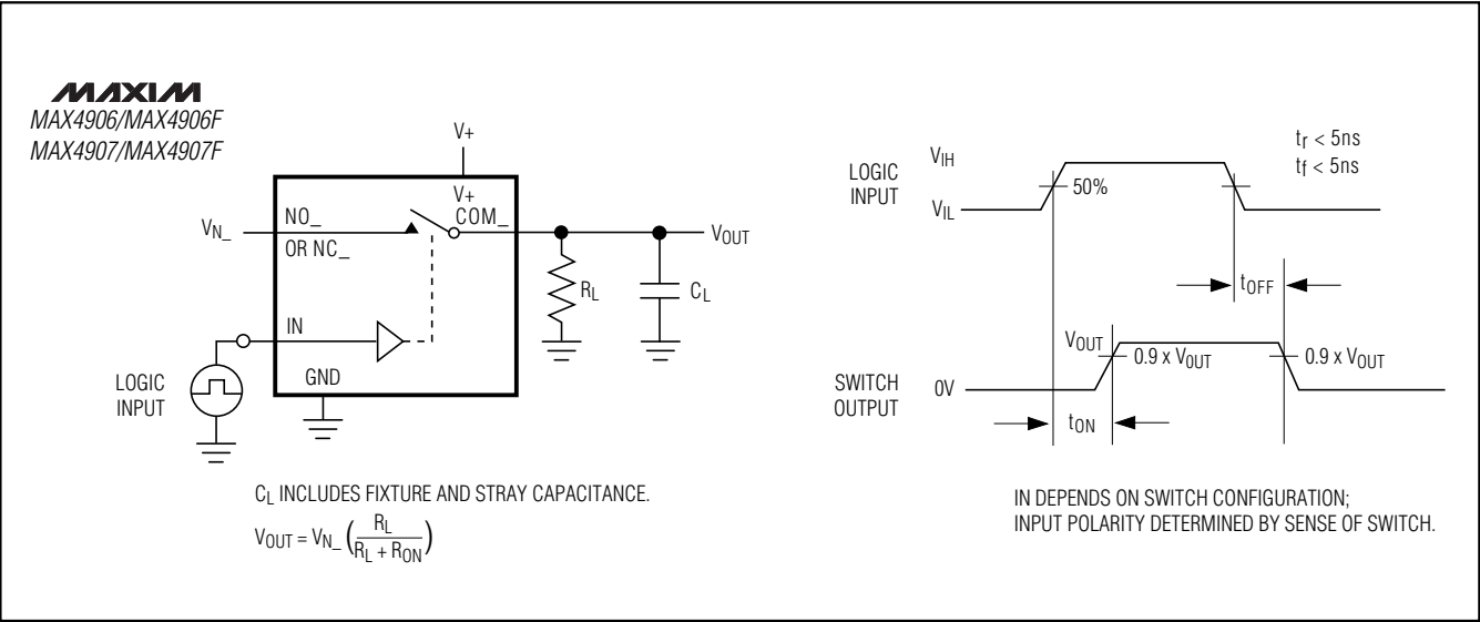
Figure 3. Switching Time
