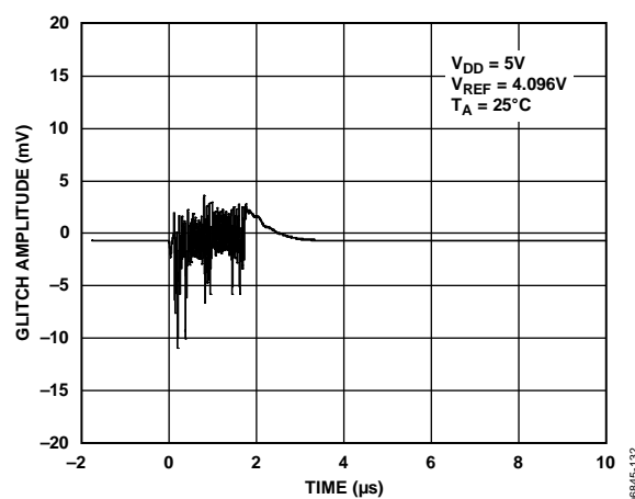
Figure 32. DAC-to-DAC Crosstalk
