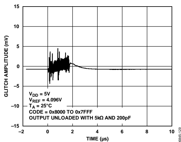
Figure 29. Glitch
